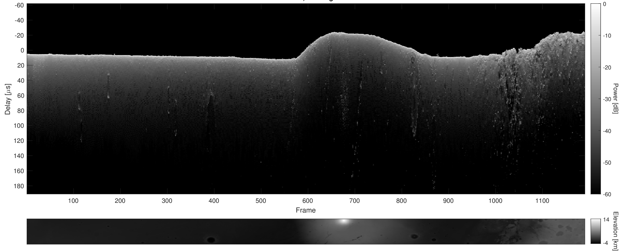
Orbit 13642, Cluttergram
