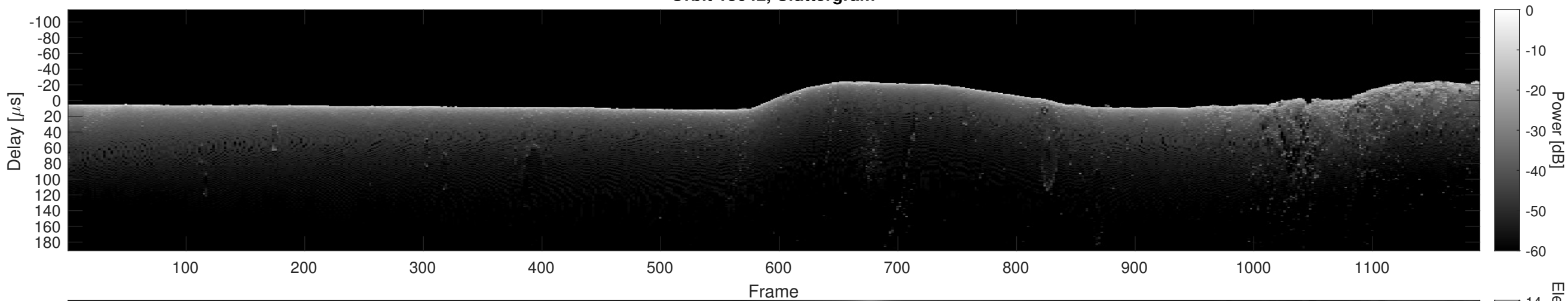
Orbit 13642, Cluttergram
