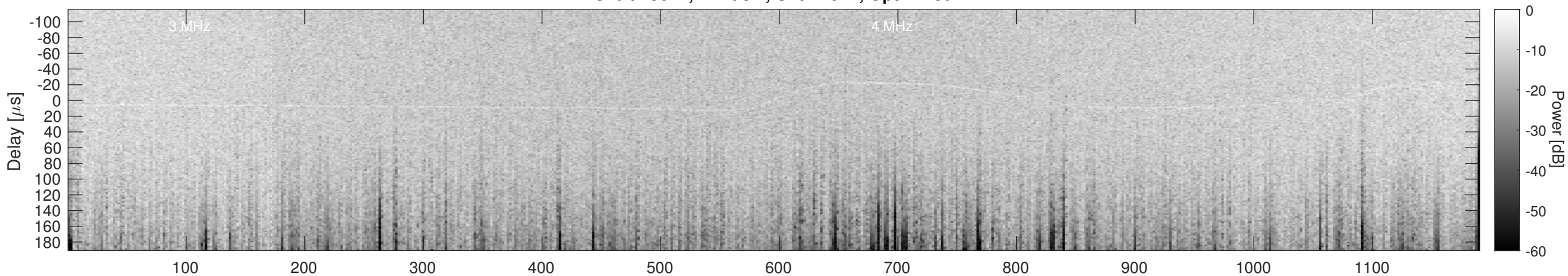
Orbit 13642, Cluttergram
