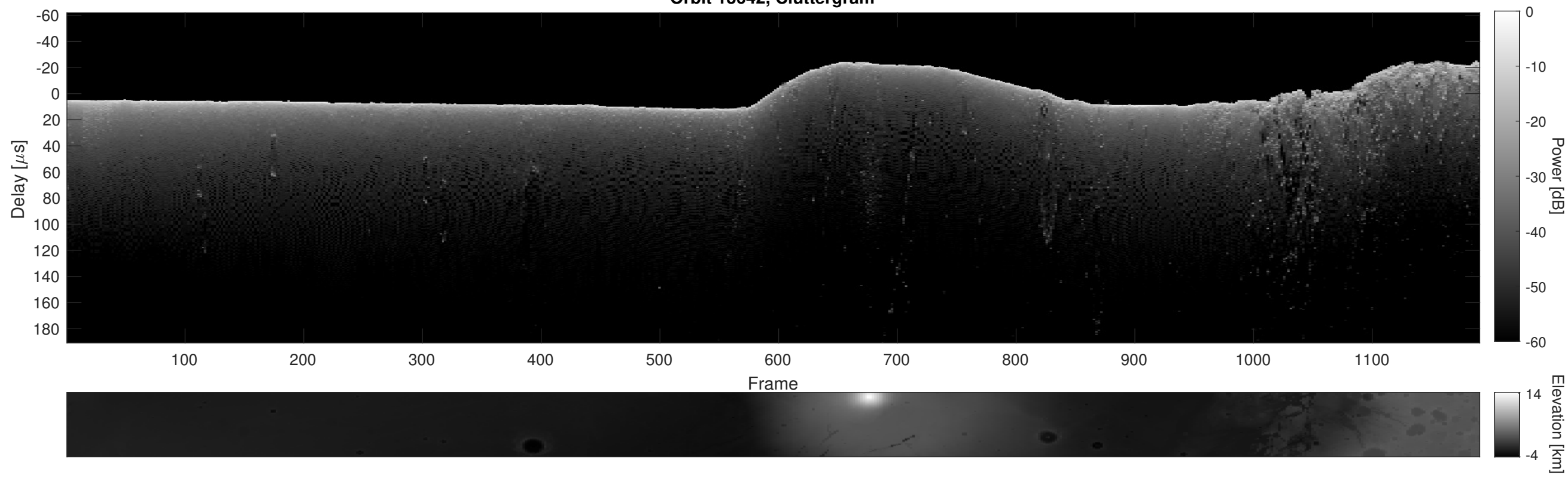
Orbit 13642, Cluttergram
