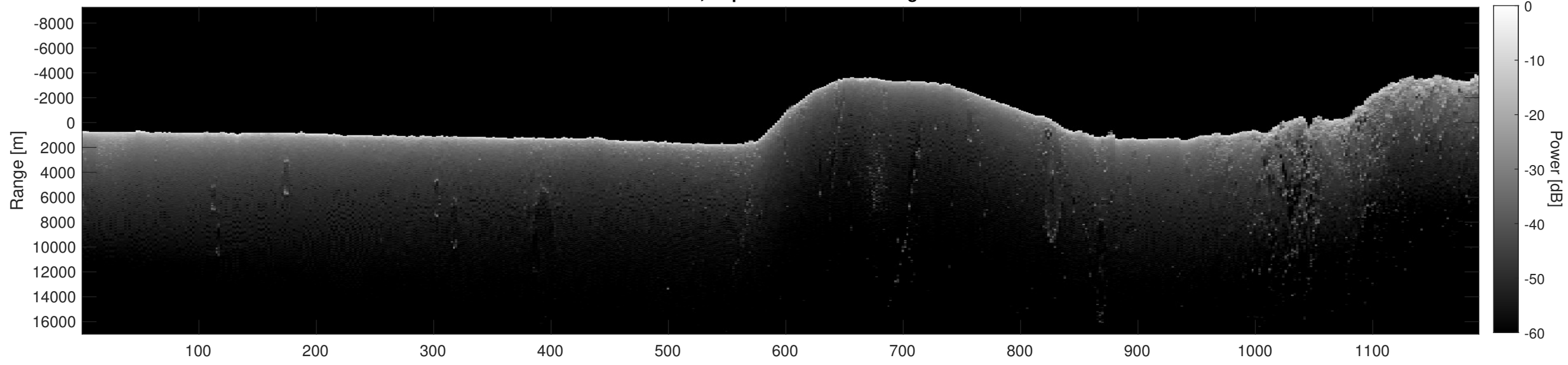
Orbit 13642, Depth-Corrected Cluttergram
