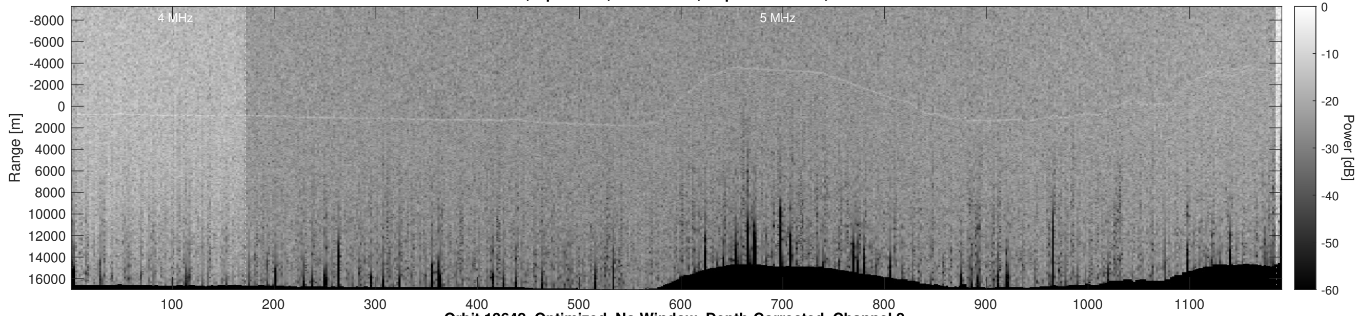
Orbit 13642, Optimized, No Window, Depth-Corrected, Channel 2
