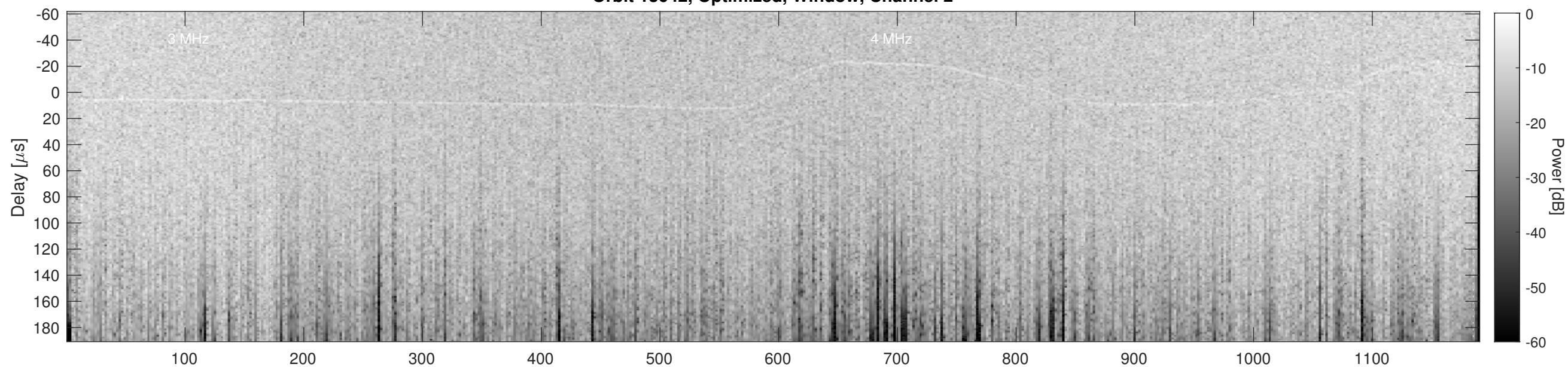
Orbit 13642, Cluttergram
