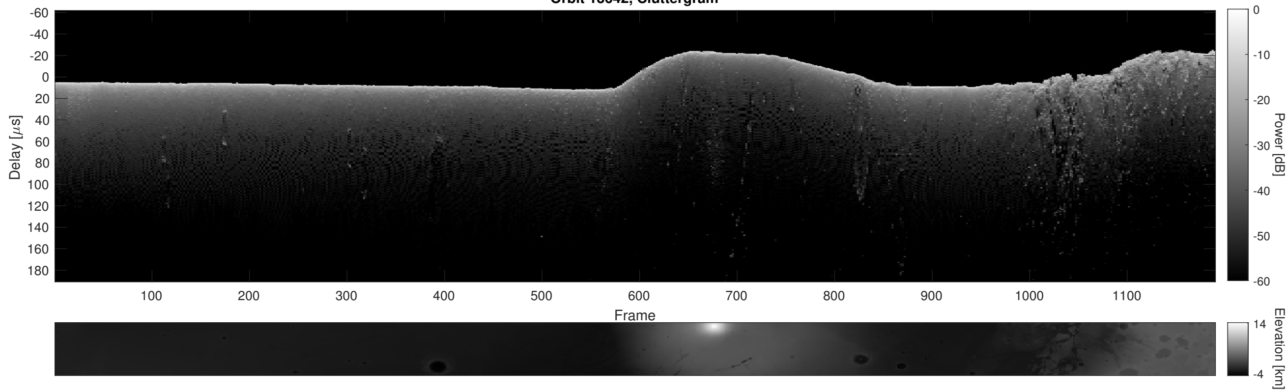
Orbit 13642, Cluttergram
