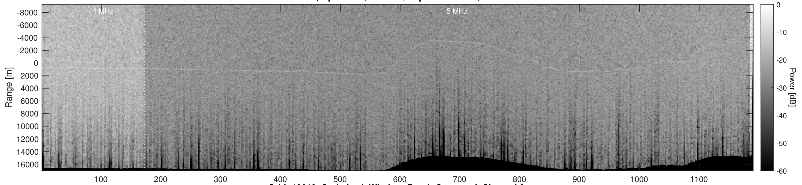
Orbit 13642, Optimized, Window, Depth-Corrected, Channel 2
