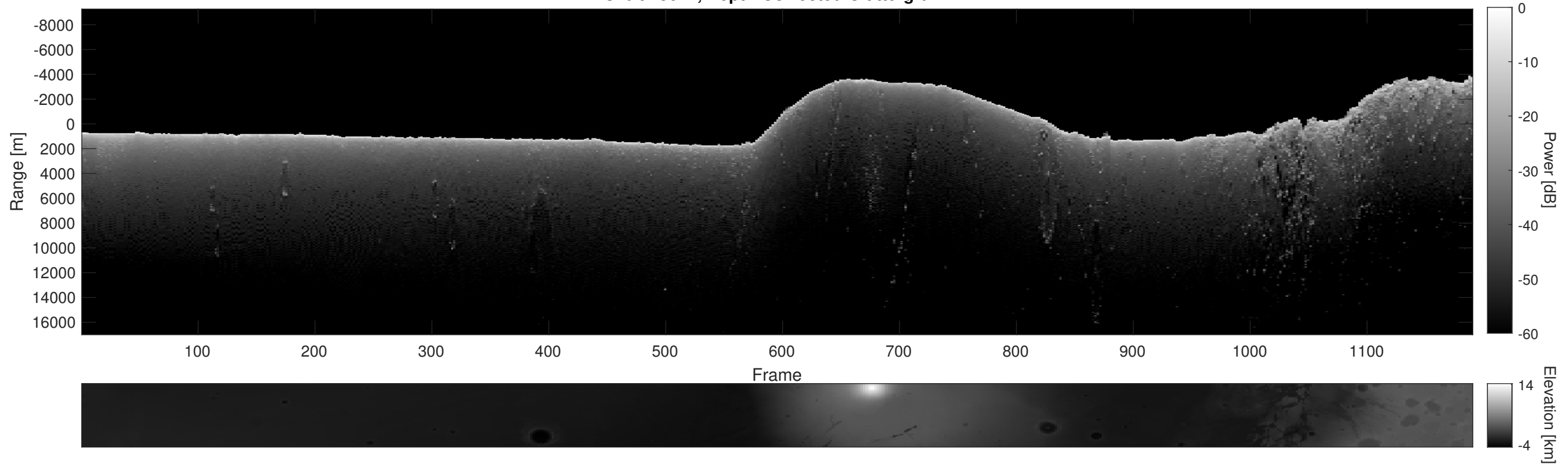
Orbit 13642, Depth-Corrected Cluttergram
