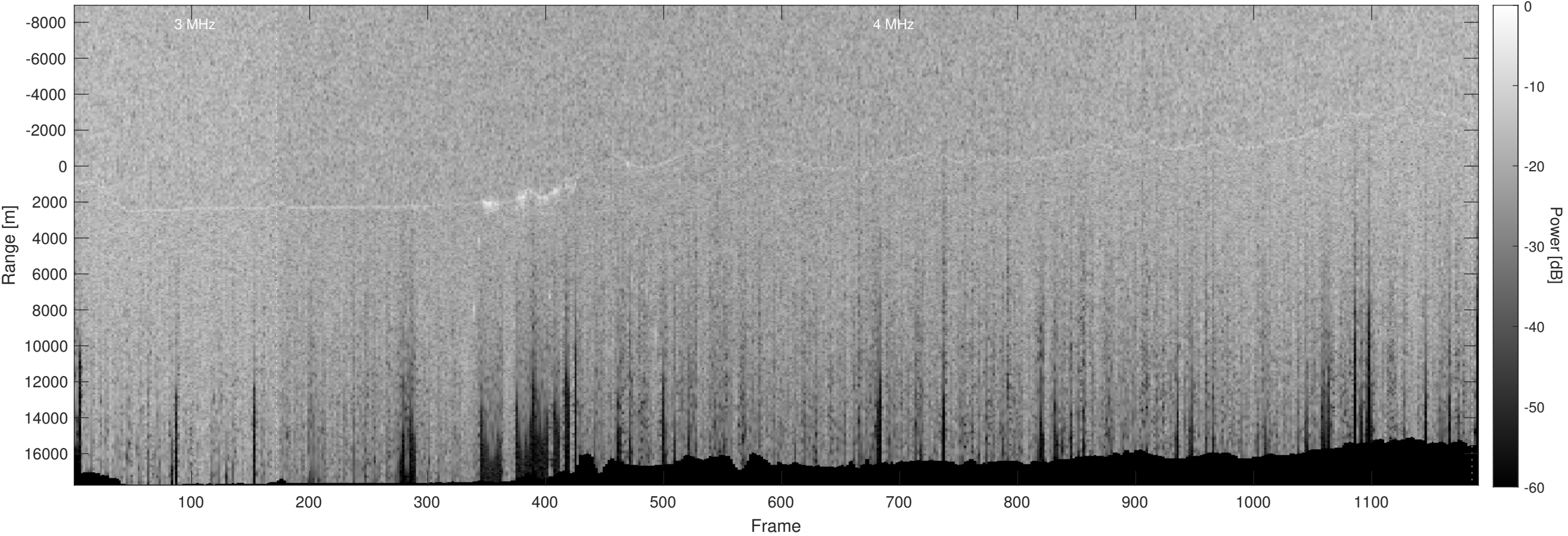
Orbit 13643, Optimized, No Window, Depth-Corrected, Channel 2
