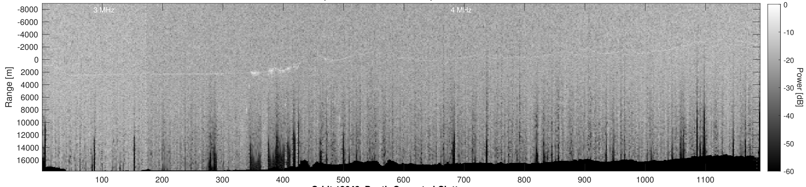
Orbit 13643, Depth-Corrected Cluttergram
