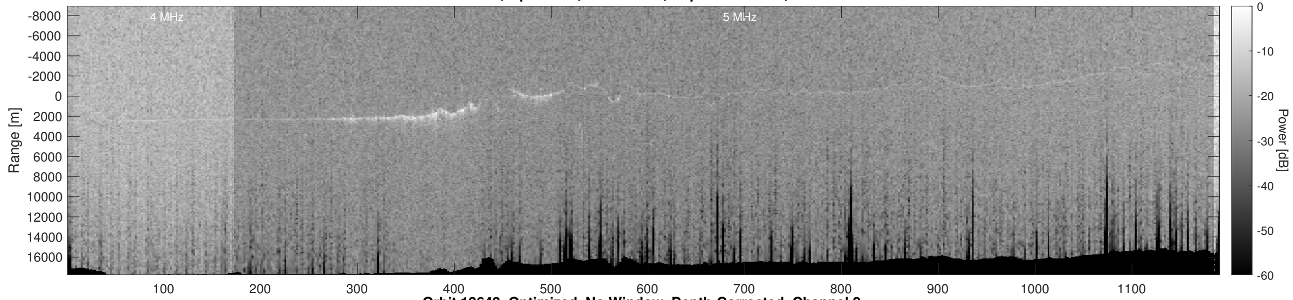
Orbit 13643, Optimized, No Window, Depth-Corrected, Channel 2
