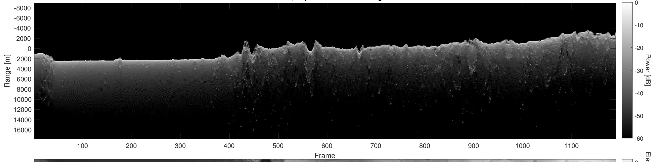
Orbit 13643, Depth-Corrected Cluttergram
