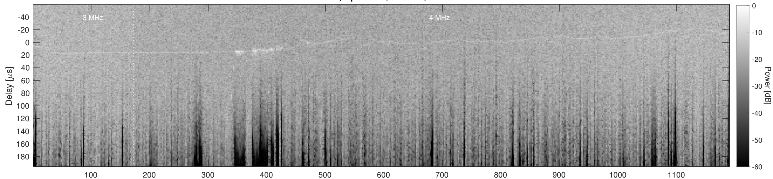
Orbit 13643, Cluttergram
