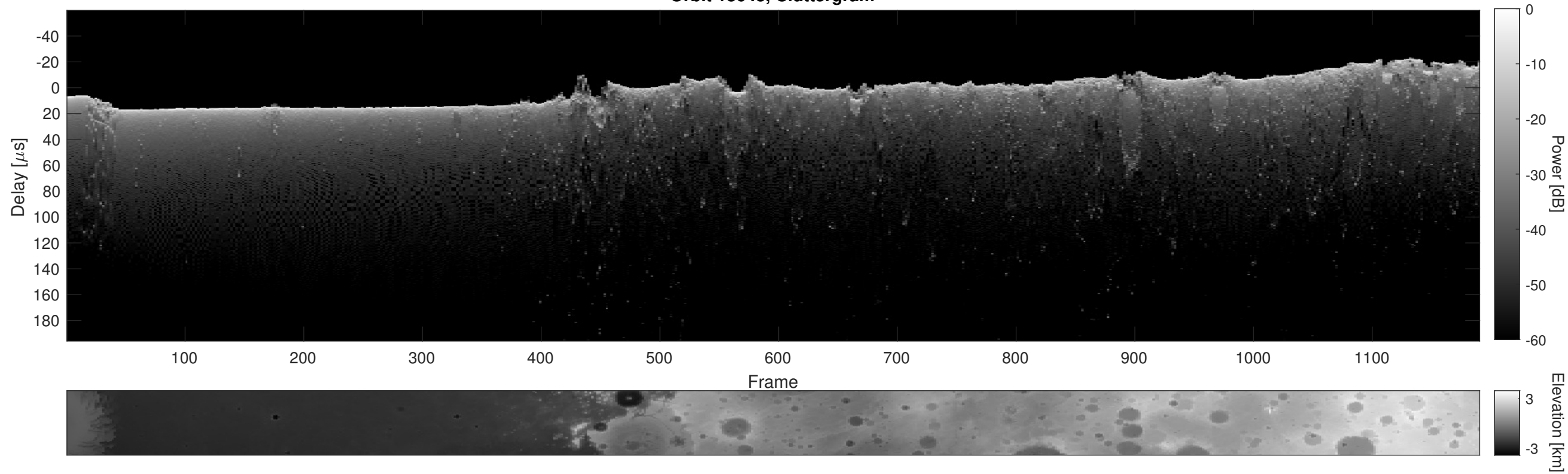
Orbit 13643, Cluttergram
