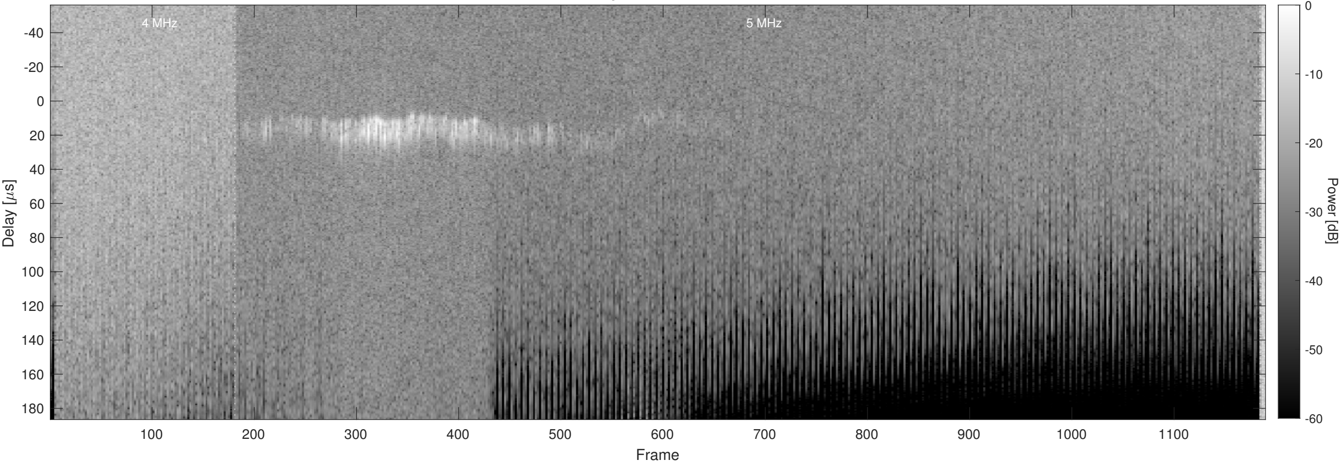
Orbit 13645, Chapman, No Window, Channel 2
