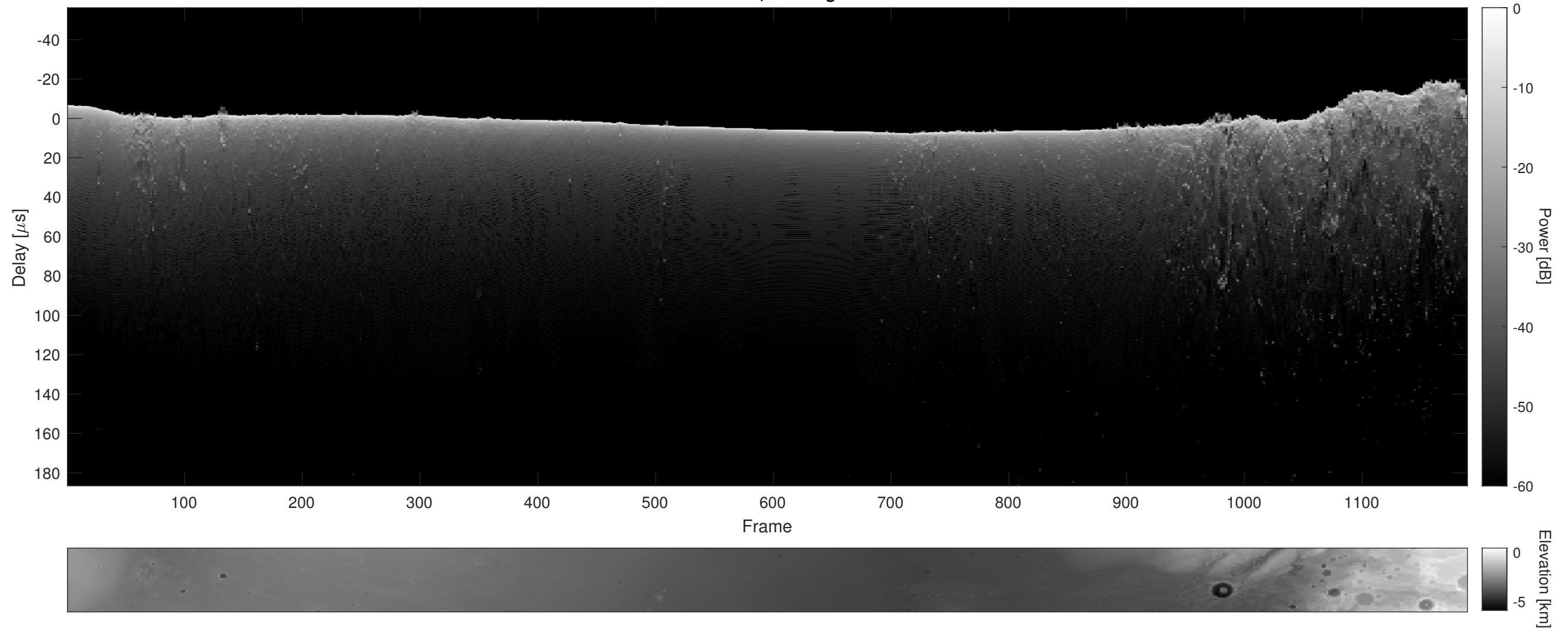
Orbit 13645, Cluttergram
