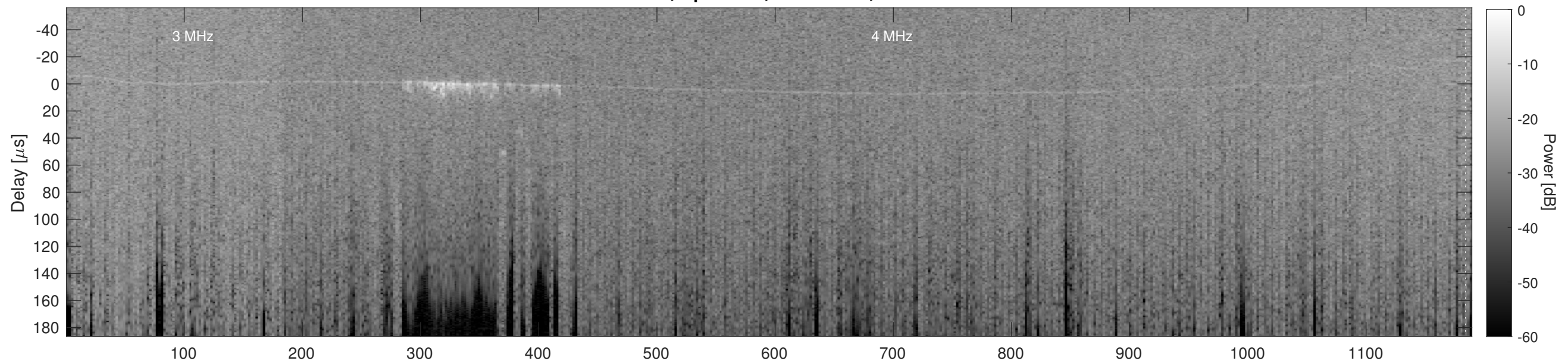
Orbit 13645, Cluttergram
