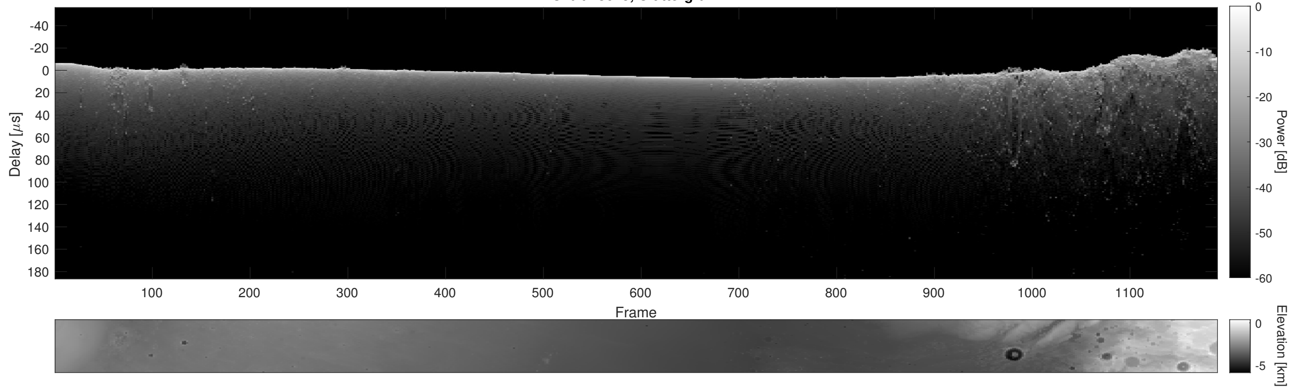
Orbit 13645, Cluttergram
