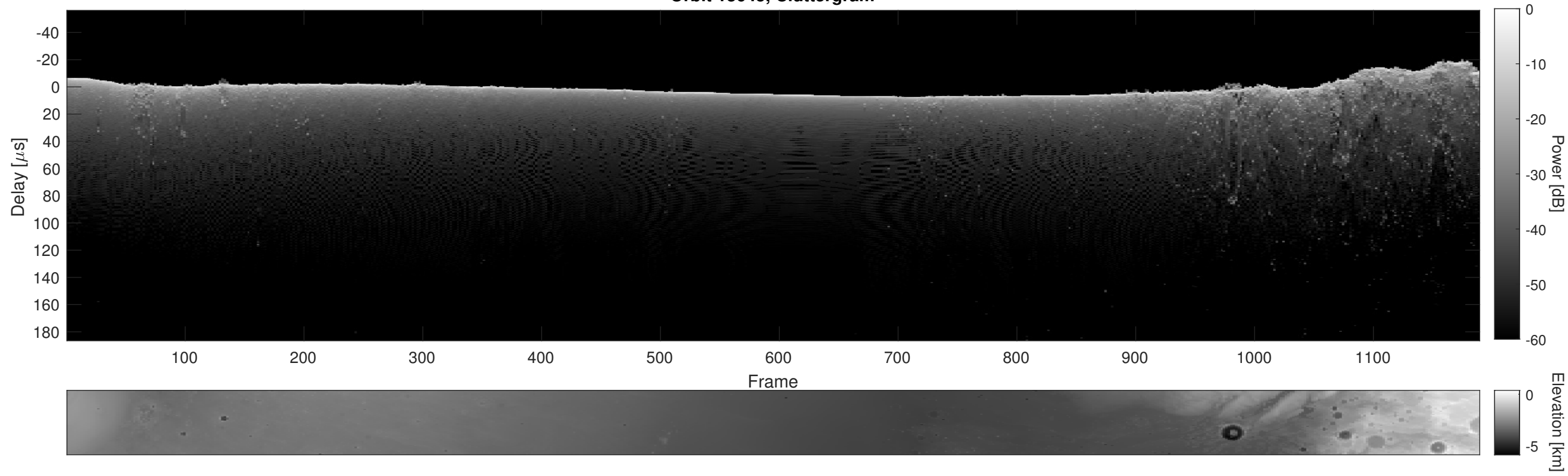
Orbit 13645, Cluttergram
