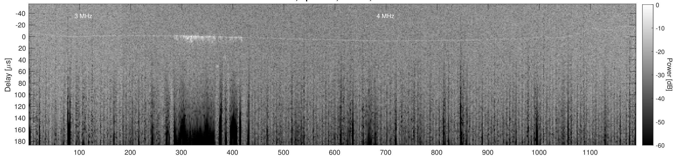
Orbit 13645, Cluttergram
