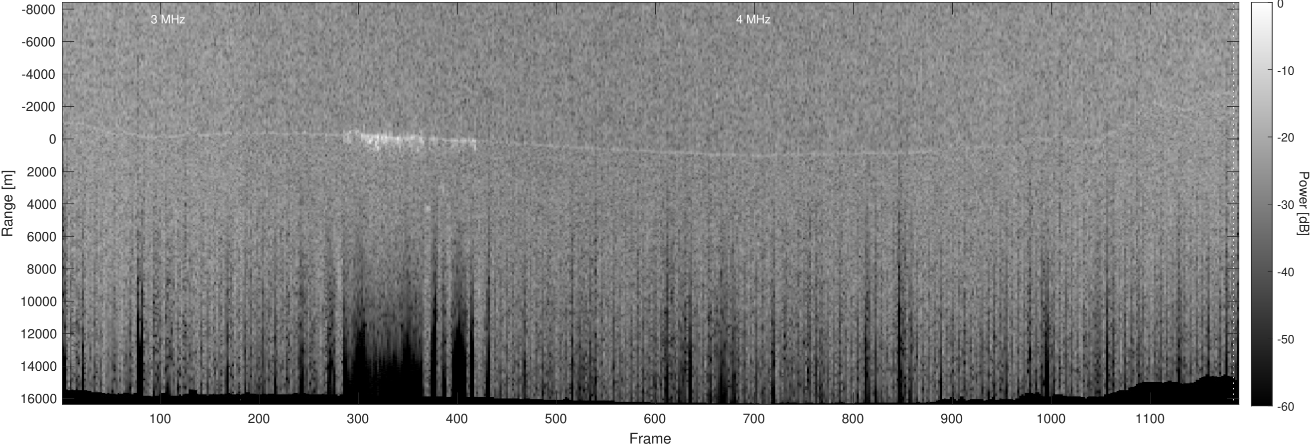
Orbit 13645, Optimized, Window, Depth-Corrected, Channel 2
