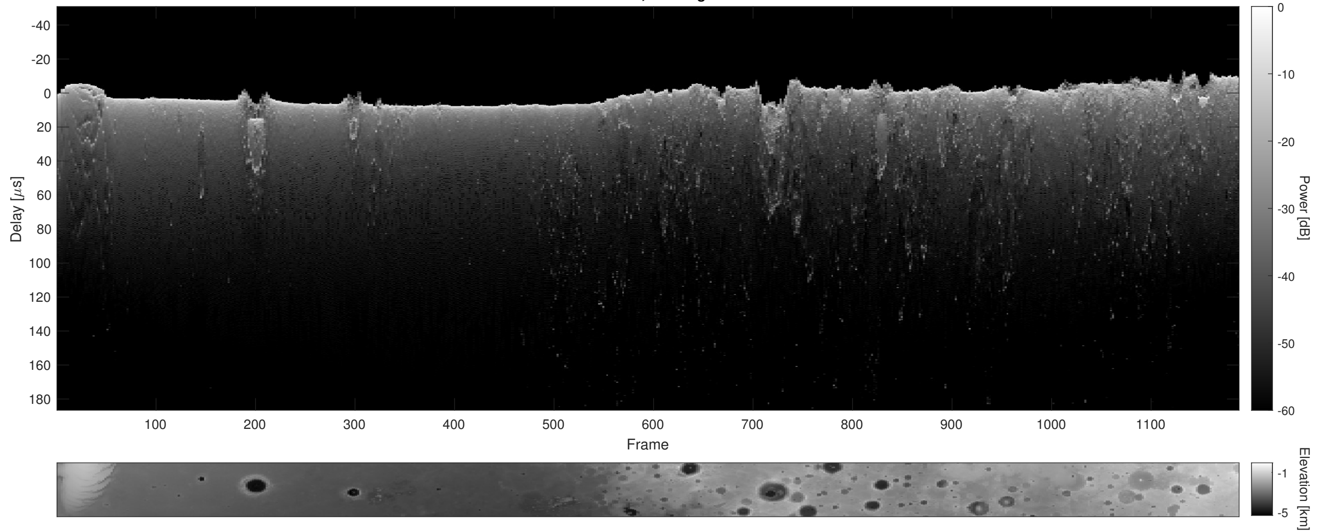
Orbit 13647, Cluttergram
