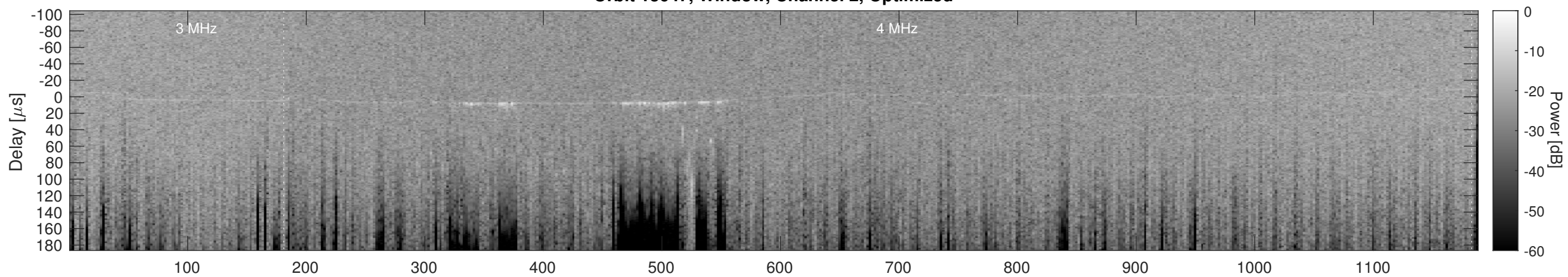
Orbit 13647, Cluttergram
