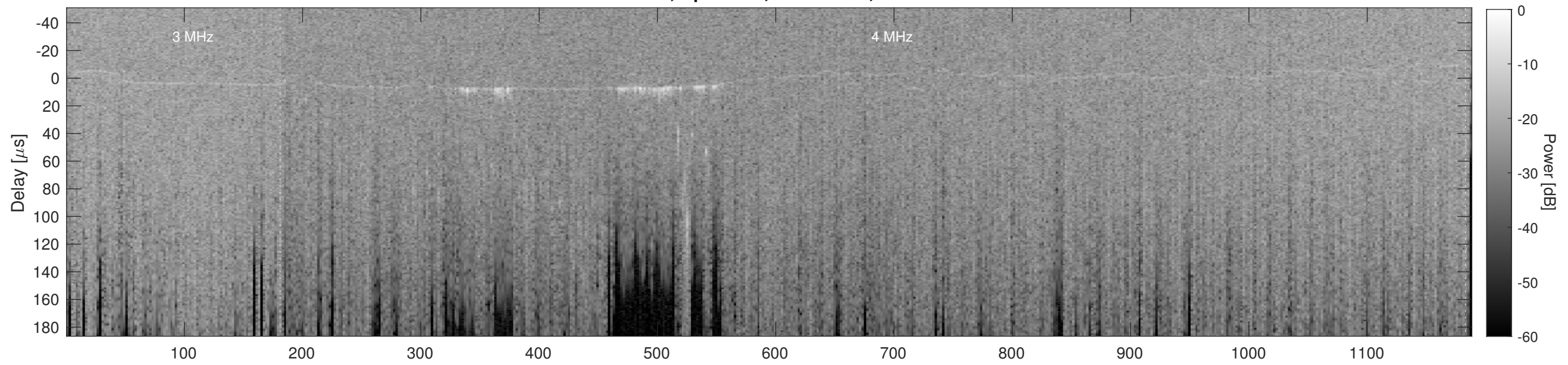
Orbit 13647, Cluttergram
