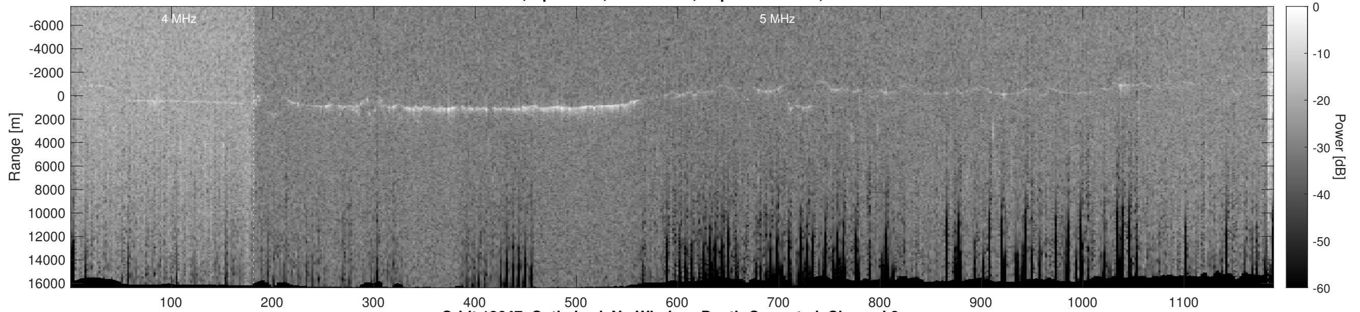
Orbit 13647, Optimized, No Window, Depth-Corrected, Channel 2
