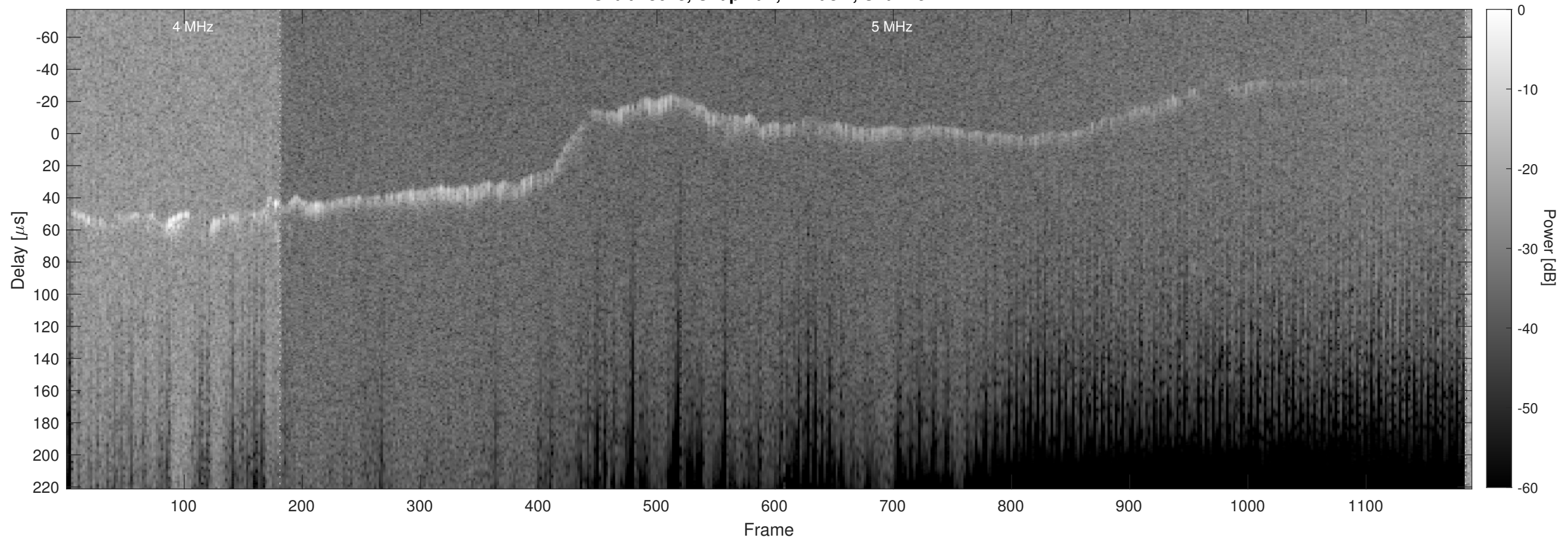
Orbit 13648, Chapman, Window, Channel 2
