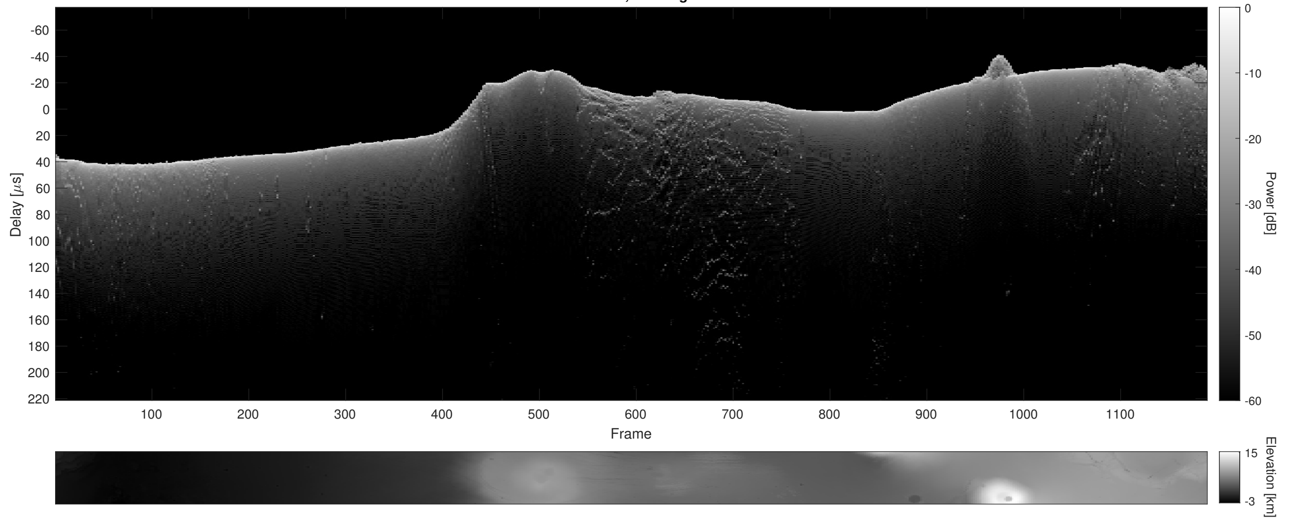
Orbit 13648, Cluttergram
