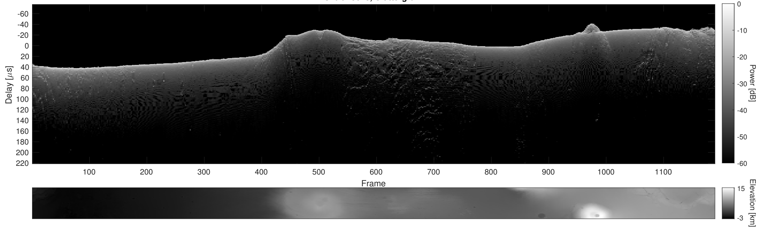
Orbit 13648, Cluttergram
