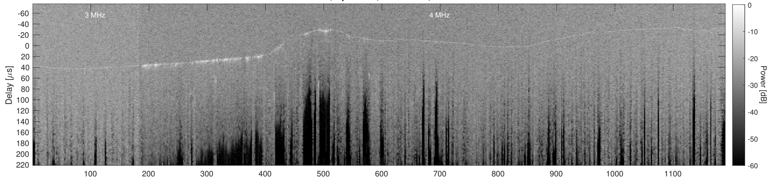
Orbit 13648, Cluttergram
