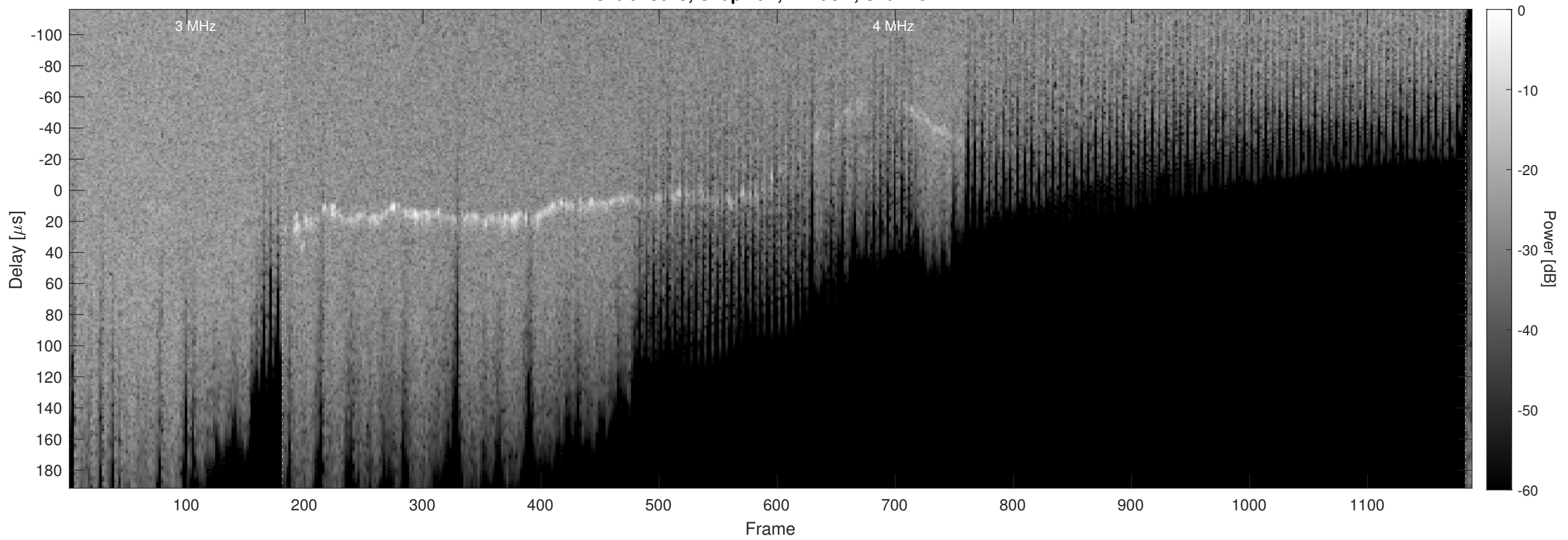
Orbit 13649, Chapman, Window, Channel 2
