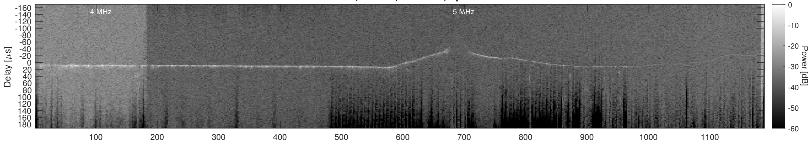
Orbit 13649, Cluttergram
