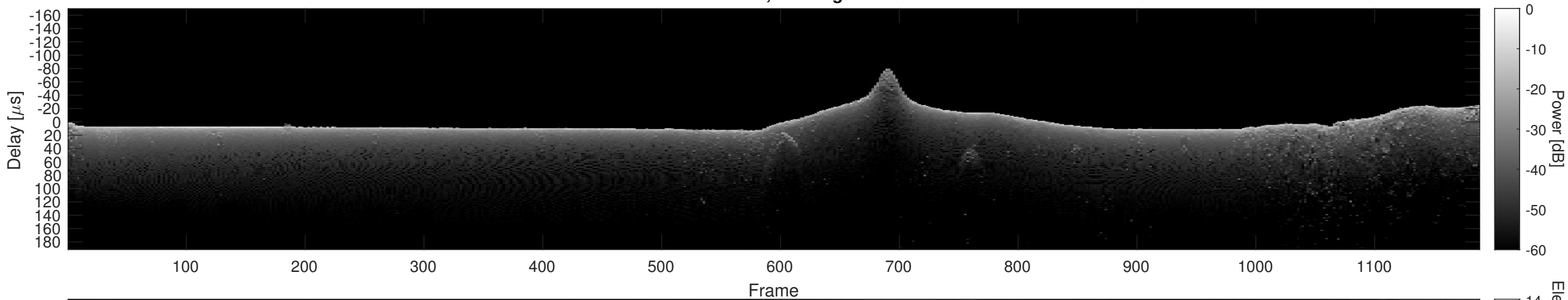
Orbit 13649, Cluttergram
