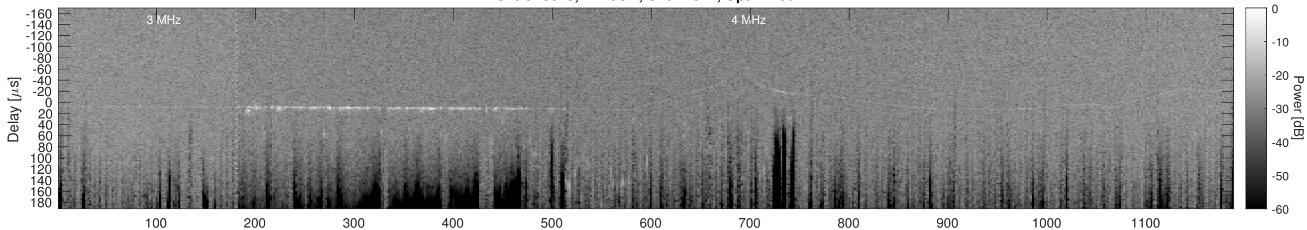
Orbit 13649, Cluttergram
