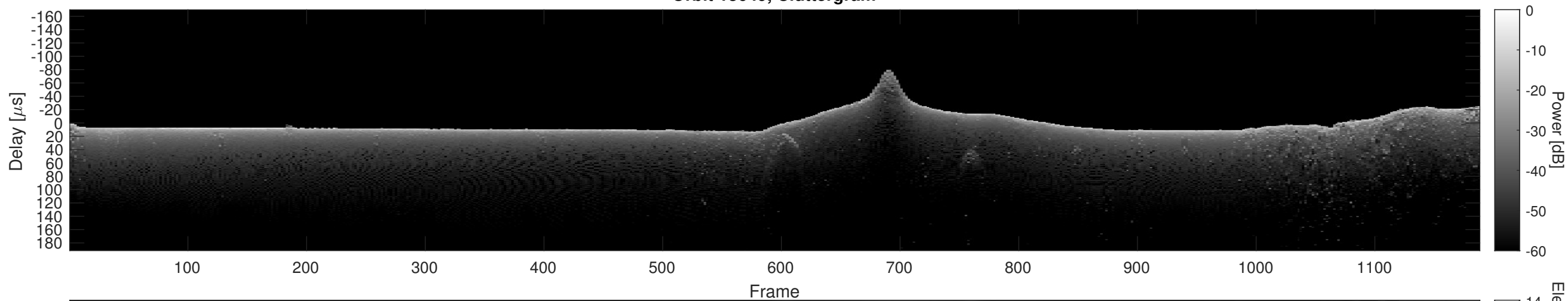
Orbit 13649, Cluttergram
