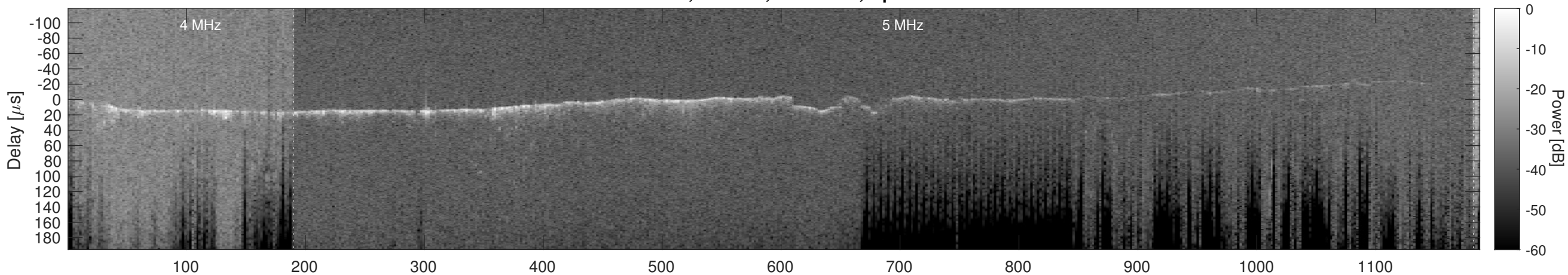
Orbit 13651, Cluttergram
