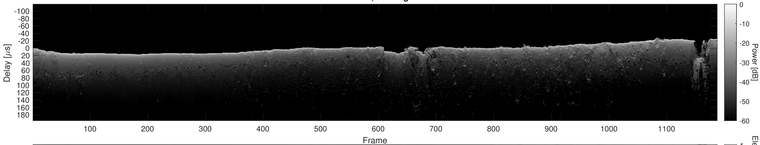
Orbit 13651, Cluttergram
