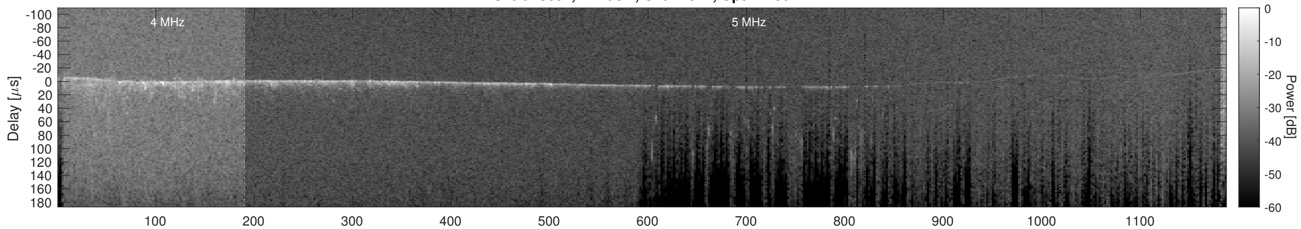
Orbit 13652, Cluttergram
