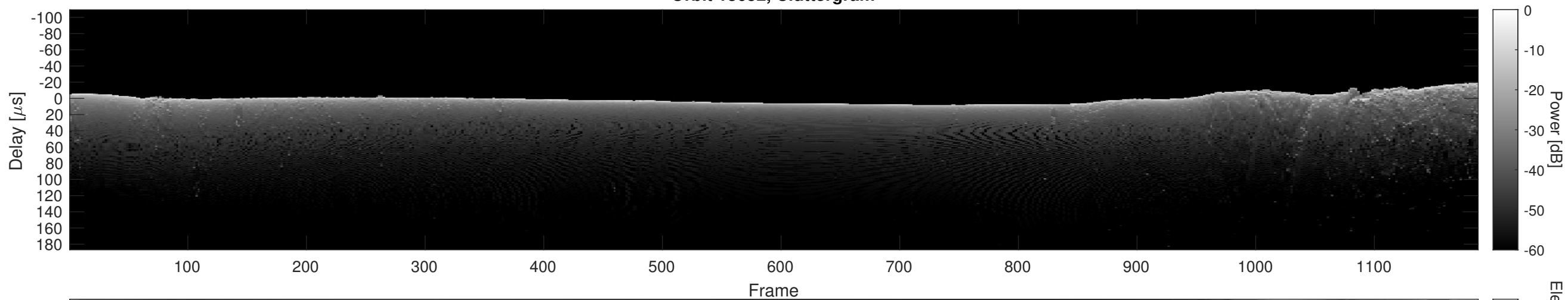
Orbit 13652, Cluttergram
