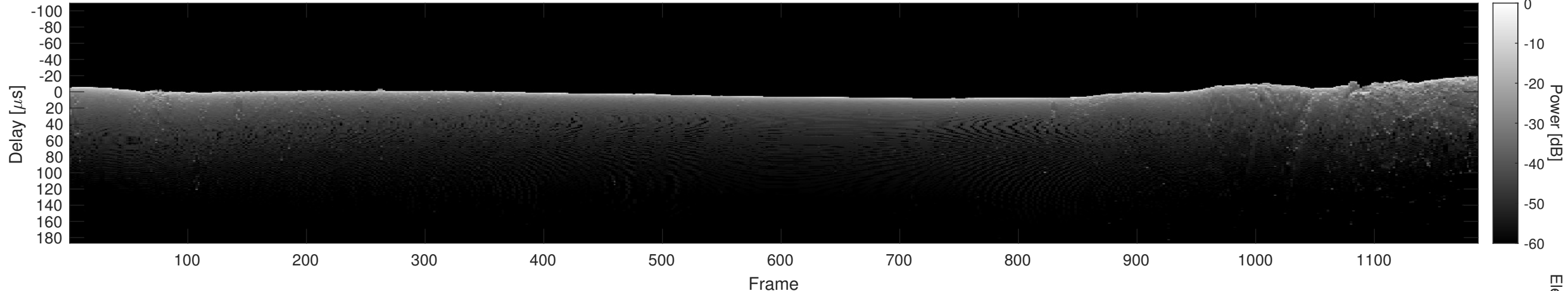
Orbit 13652, Cluttergram
