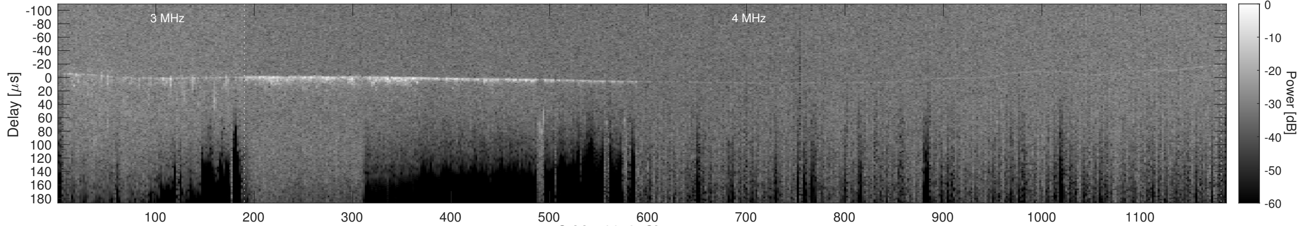
Orbit 13652, Cluttergram
