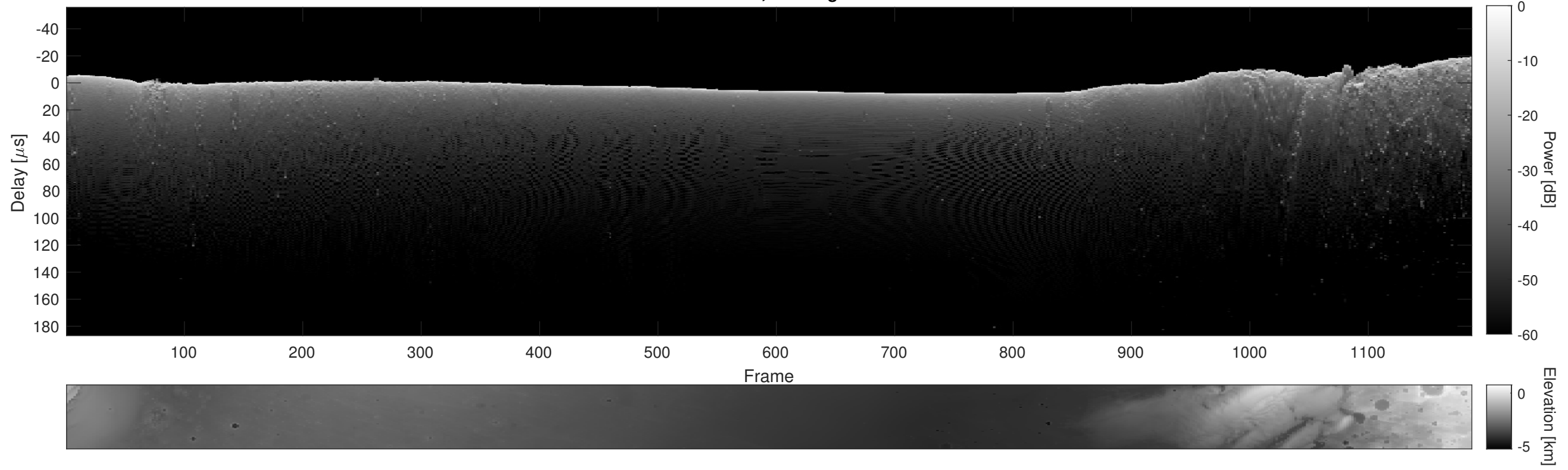
Orbit 13652, Cluttergram
