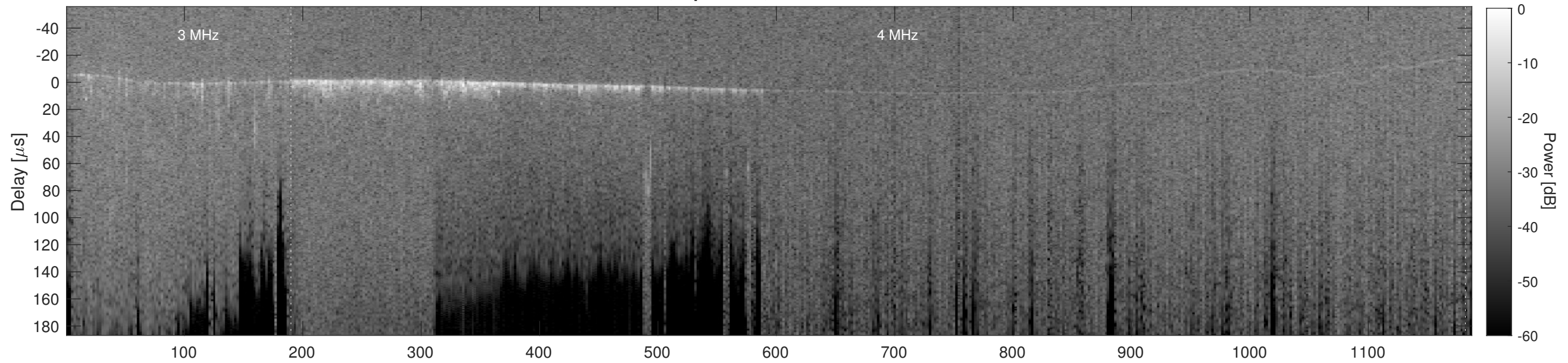
Orbit 13652, Cluttergram
