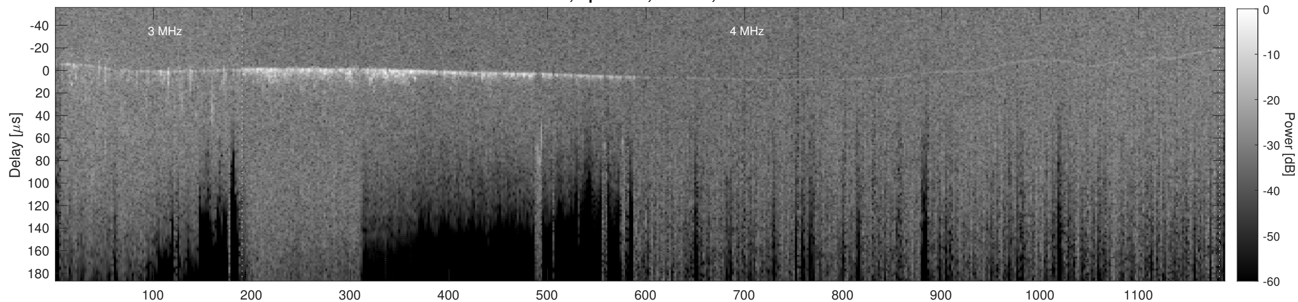
Orbit 13652, Cluttergram
