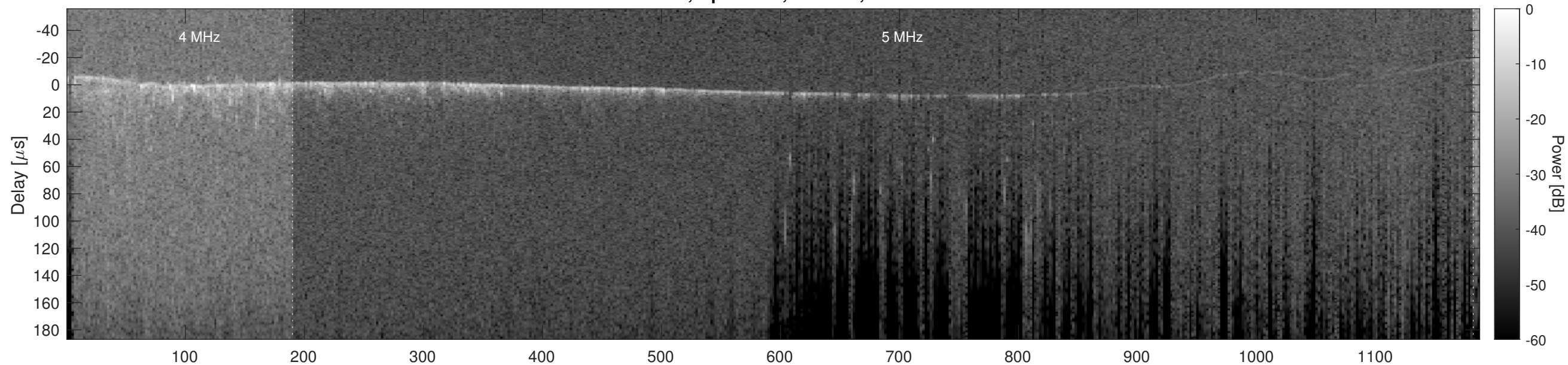
Orbit 13652, Optimized, Window, Channel 2
