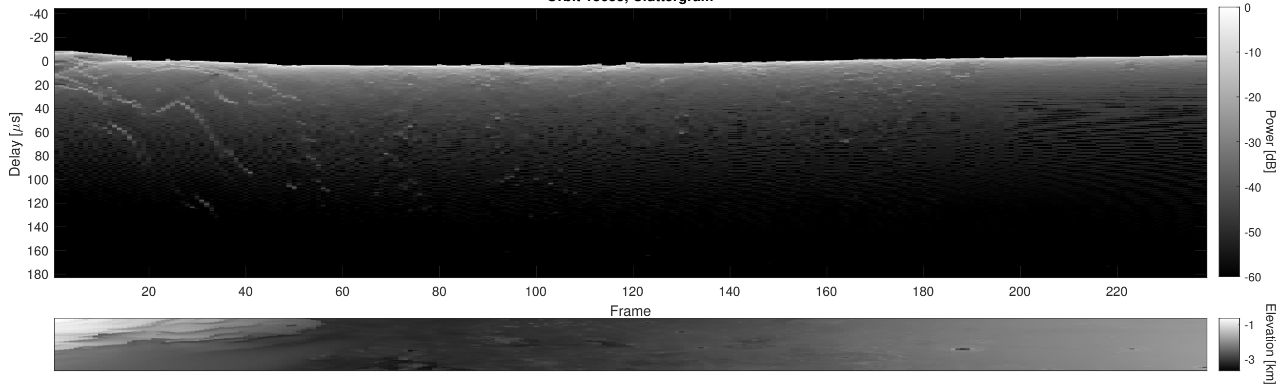
Orbit 13655, Cluttergram
