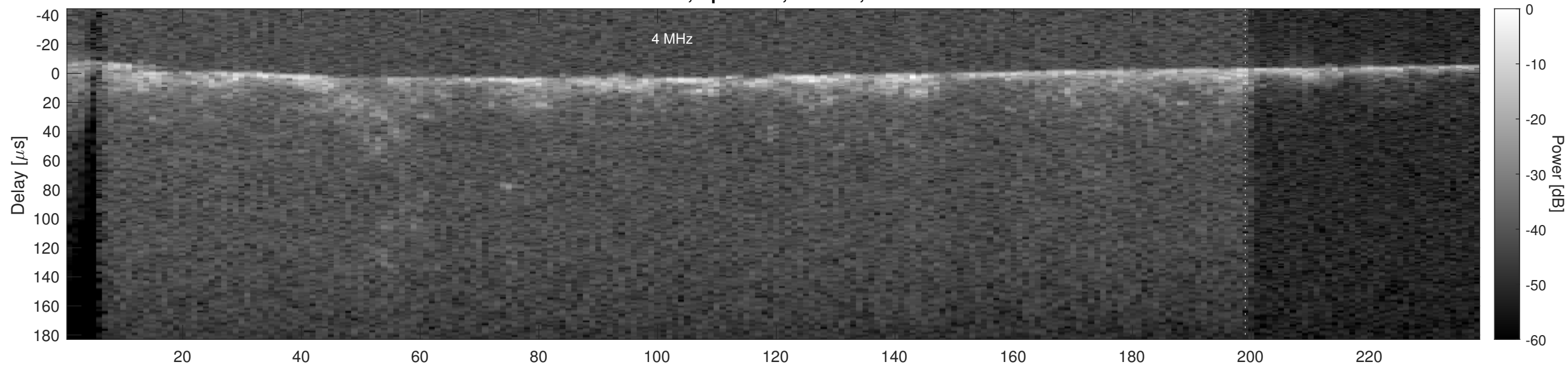
Orbit 13655, Optimized, Window, Channel 2
