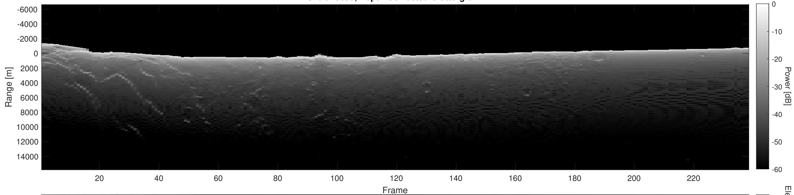
Orbit 13655, Depth-Corrected Cluttergram
