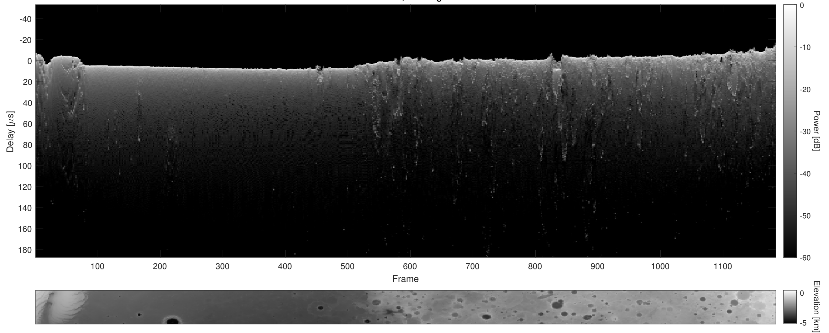
Orbit 13661, Cluttergram
