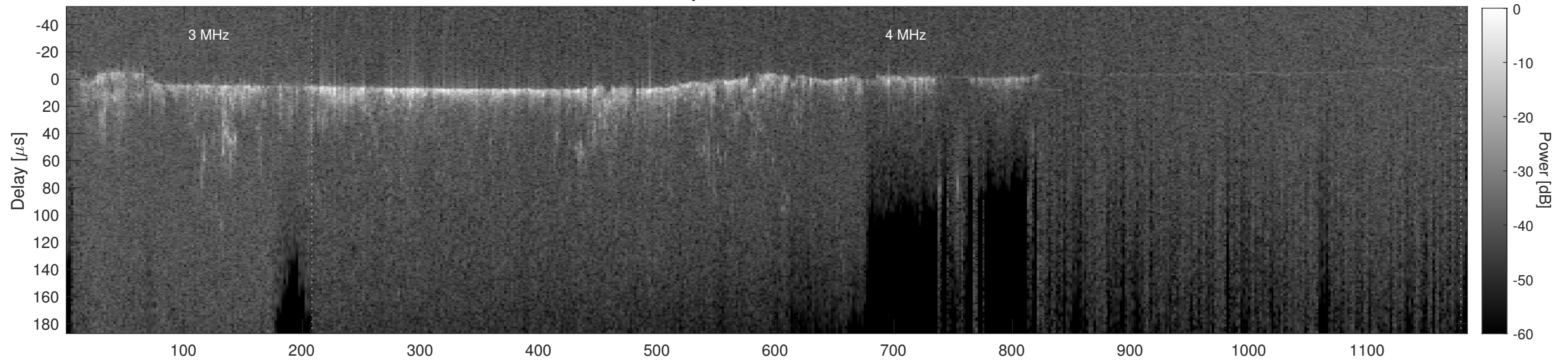
Orbit 13661, Cluttergram
