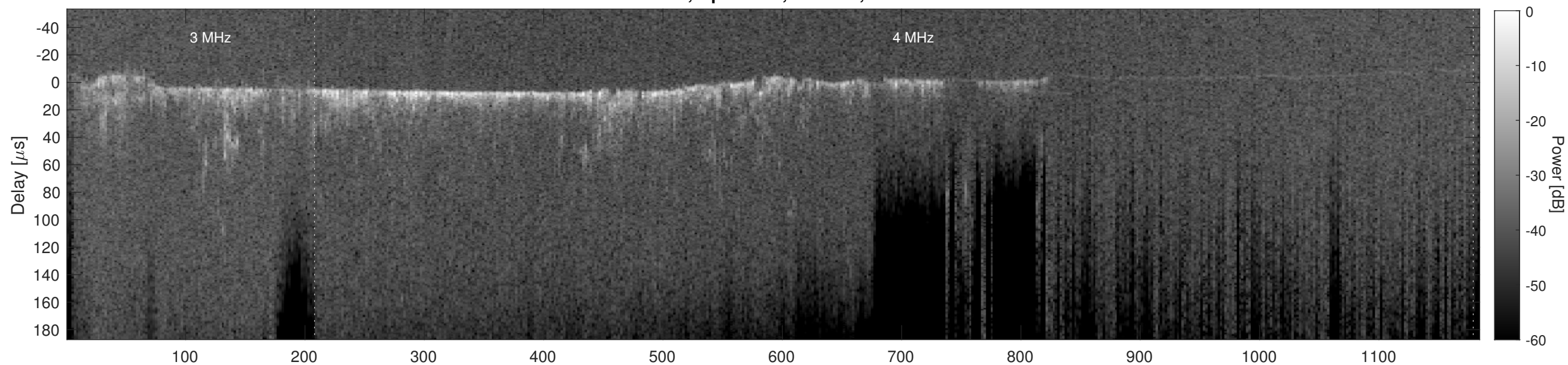
Orbit 13661, Cluttergram
