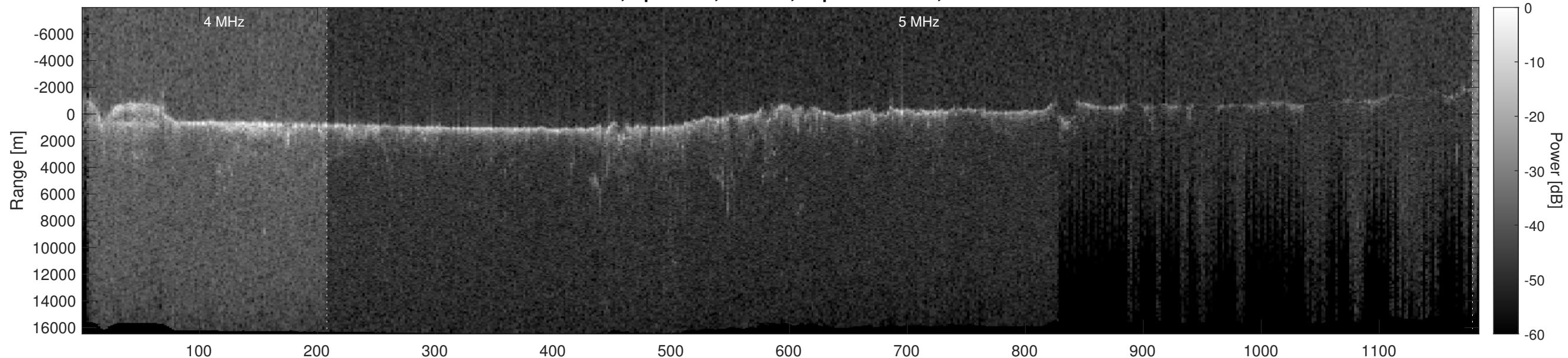
Orbit 13661, Optimized, Window, Depth-Corrected, Channel 2
