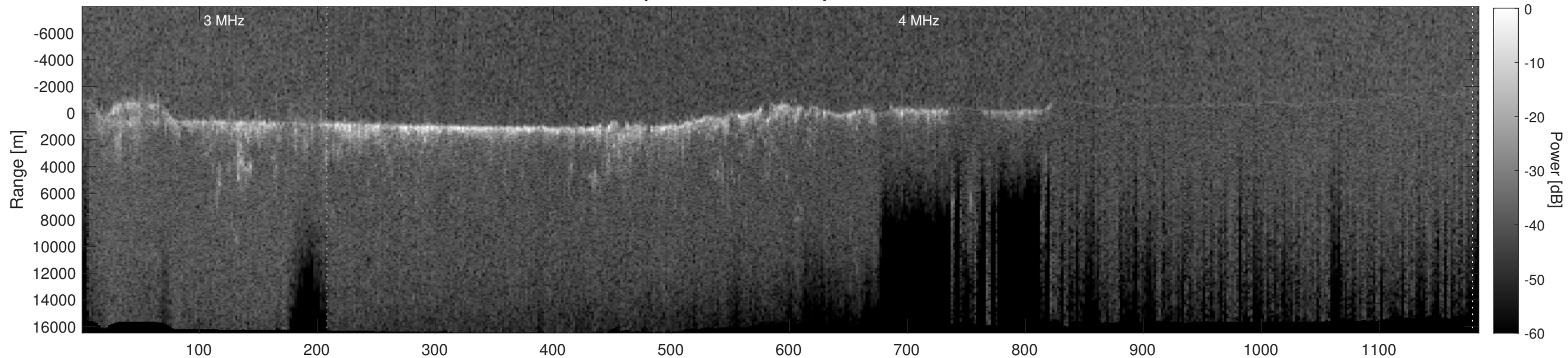
Orbit 13661, Depth-Corrected Cluttergram
