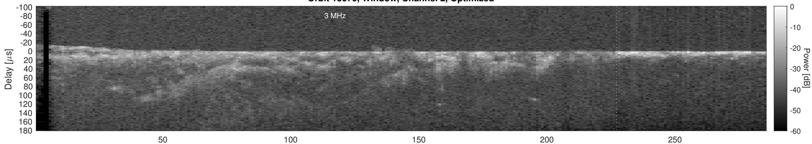
Orbit 13670, Cluttergram
