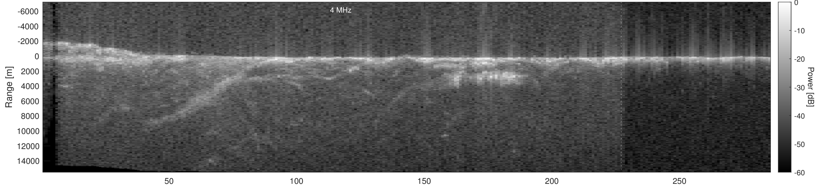
Orbit 13670, Optimized, No Window, Depth-Corrected, Channel 2
