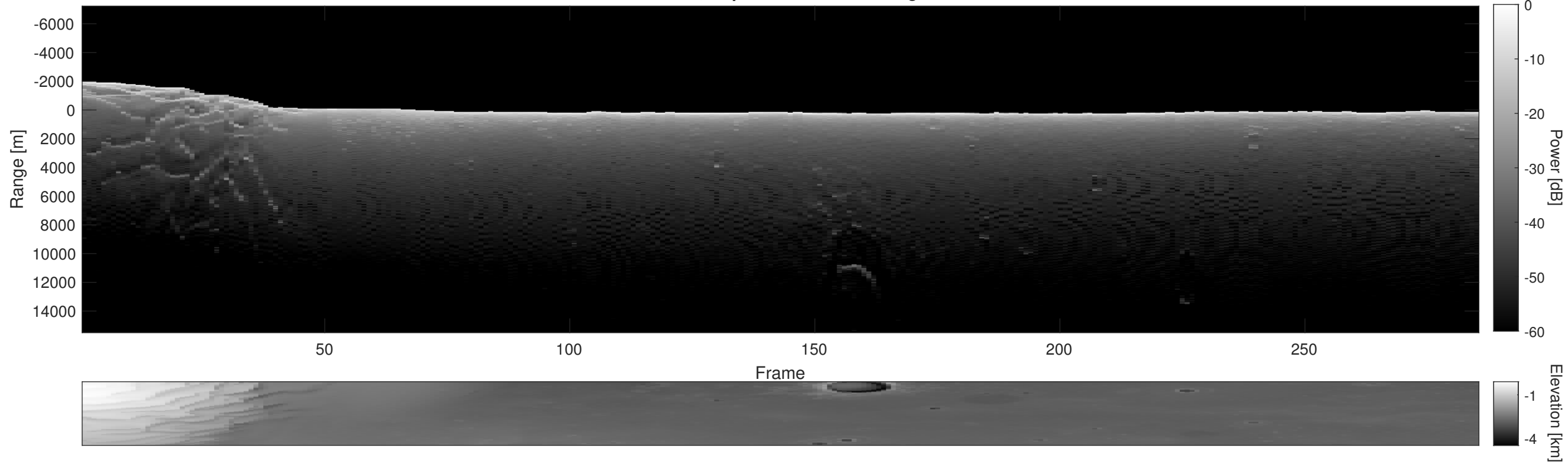
Orbit 13670, Depth-Corrected Cluttergram
