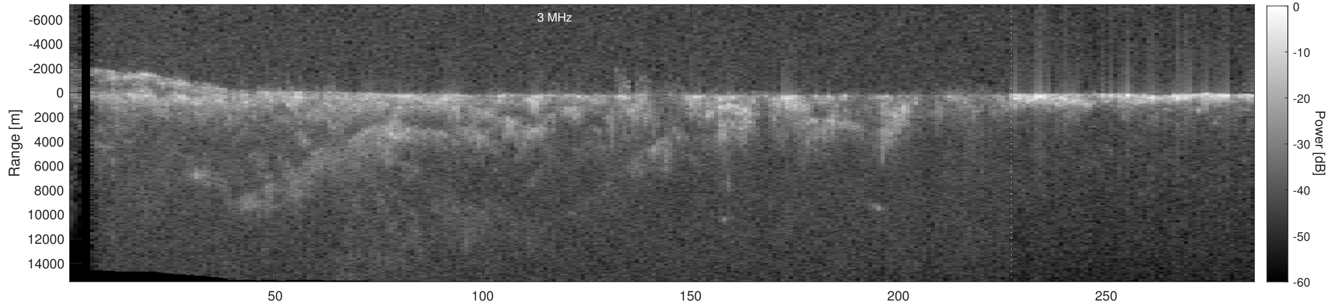
Orbit 13670, Depth-Corrected Cluttergram
