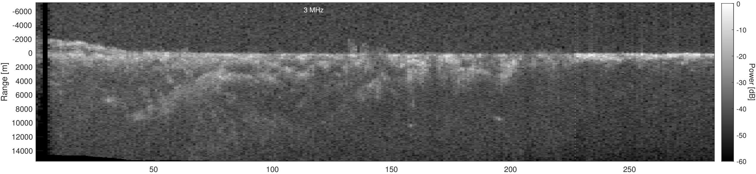
Orbit 13670, Depth-Corrected Cluttergram
