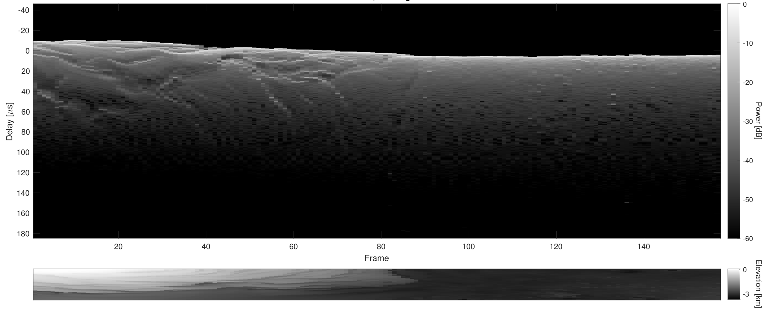
Orbit 13676, Cluttergram
