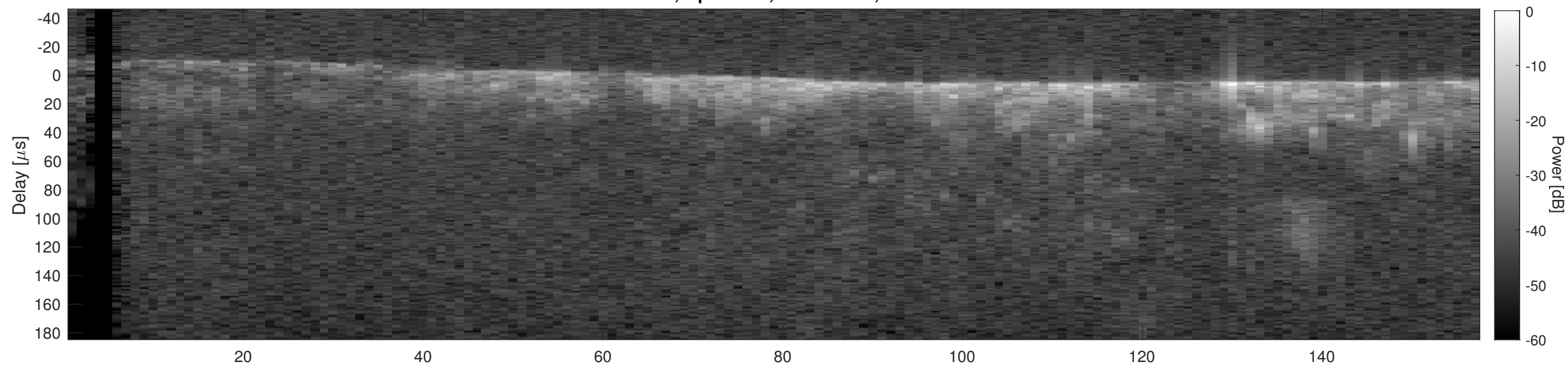
Orbit 13676, Cluttergram
