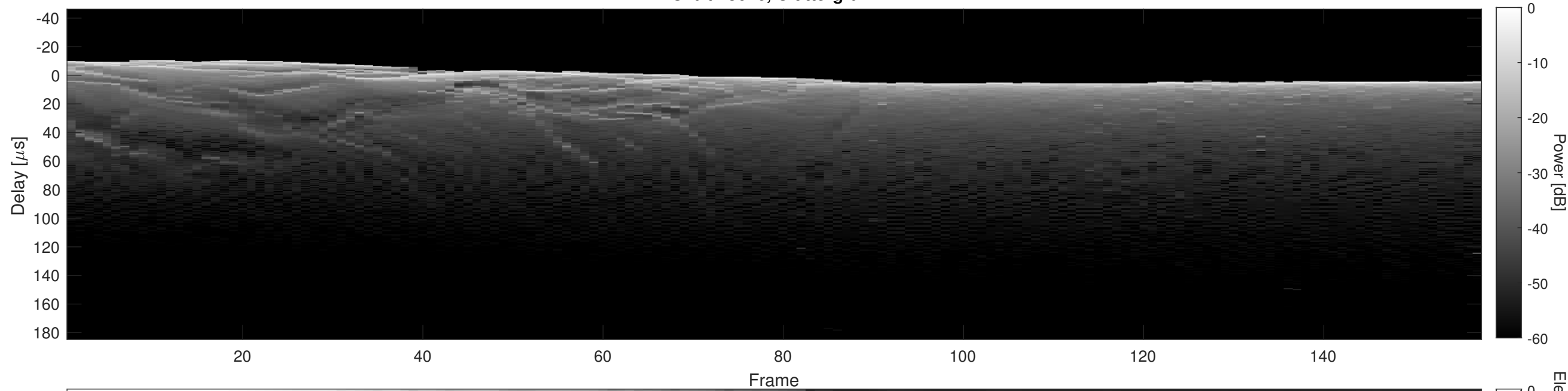
Orbit 13676, Cluttergram
