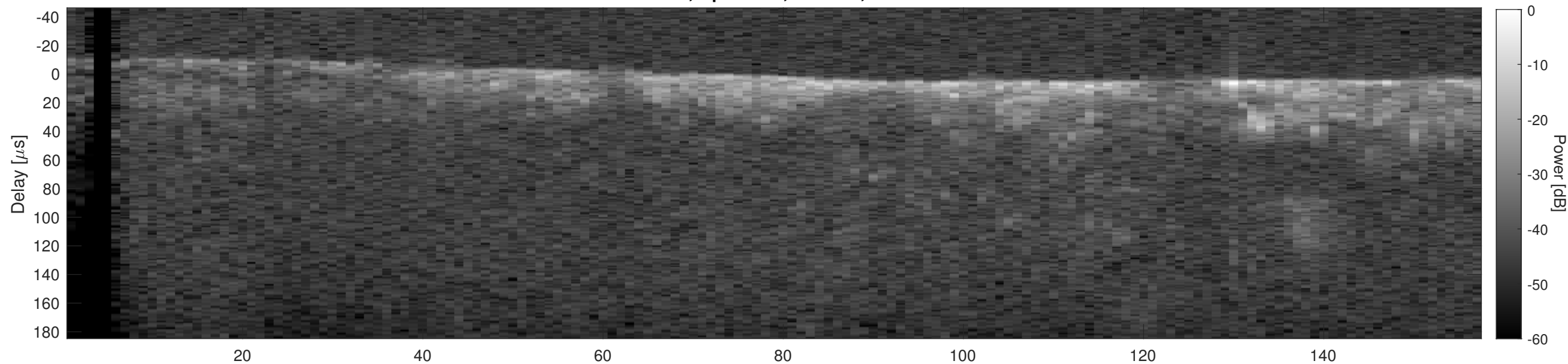
Orbit 13676, Cluttergram
