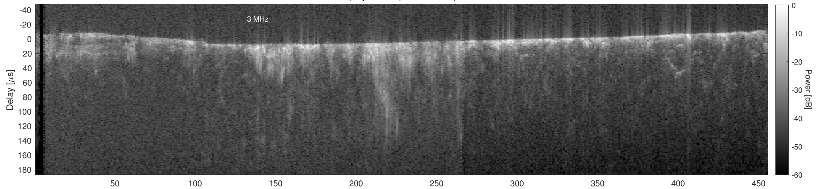
Orbit 13690, Cluttergram
