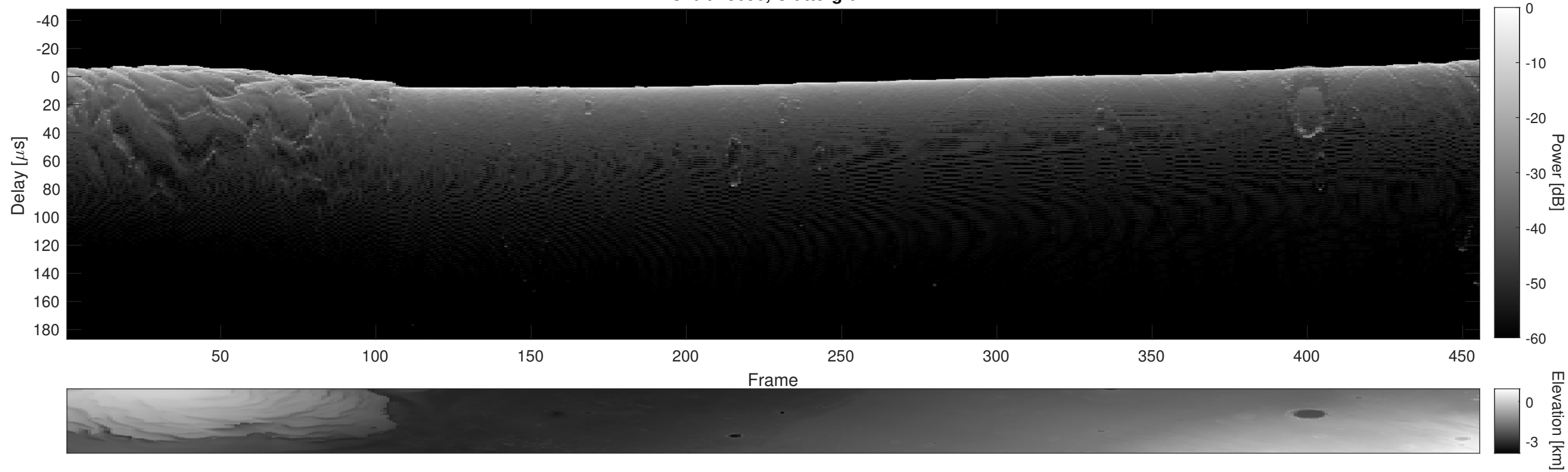
Orbit 13690, Cluttergram
