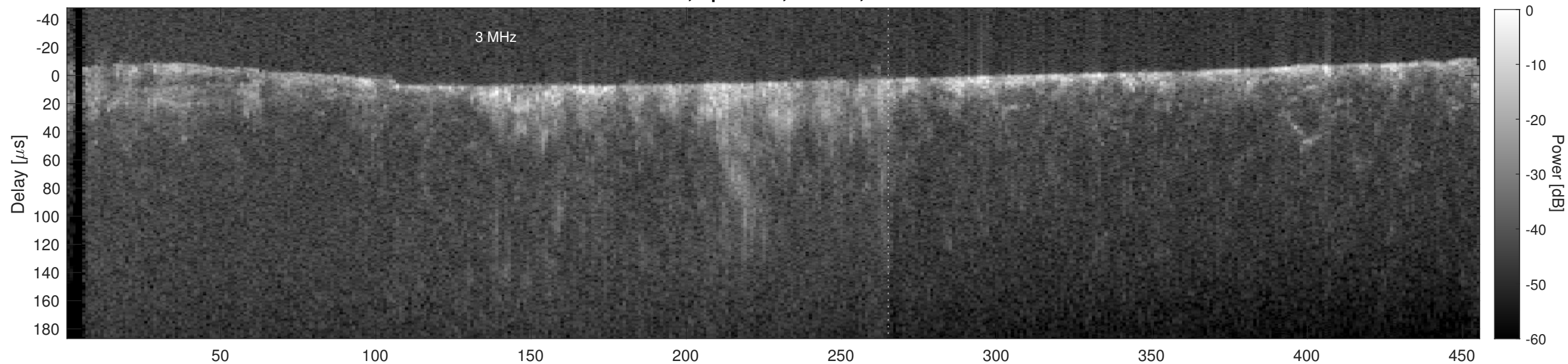
Orbit 13690, Cluttergram
