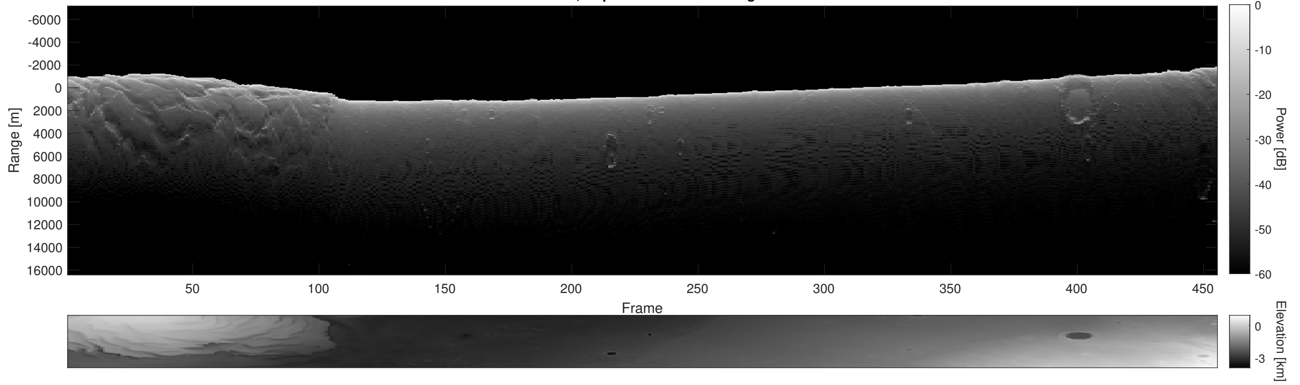
Orbit 13690, Depth-Corrected Cluttergram
