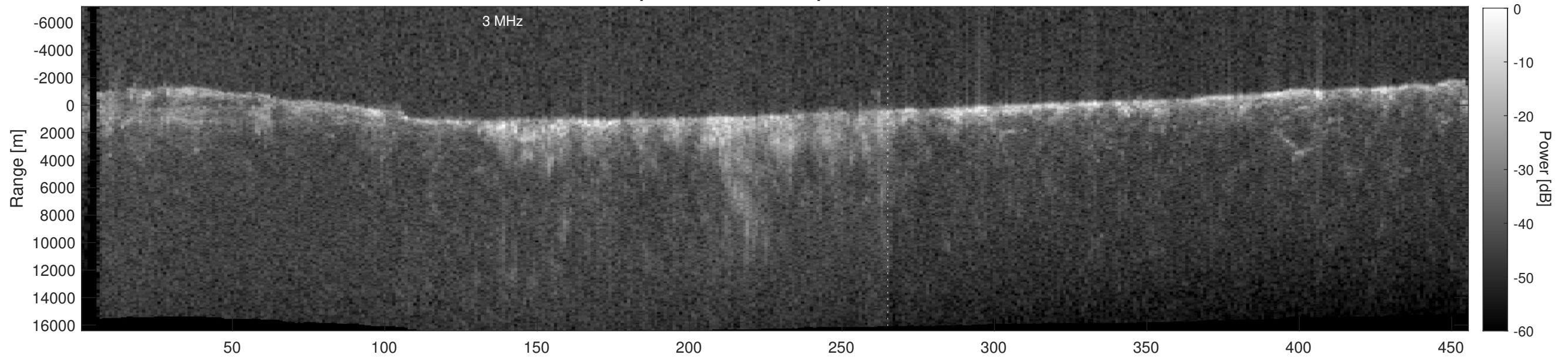
Orbit 13690, Depth-Corrected Cluttergram
