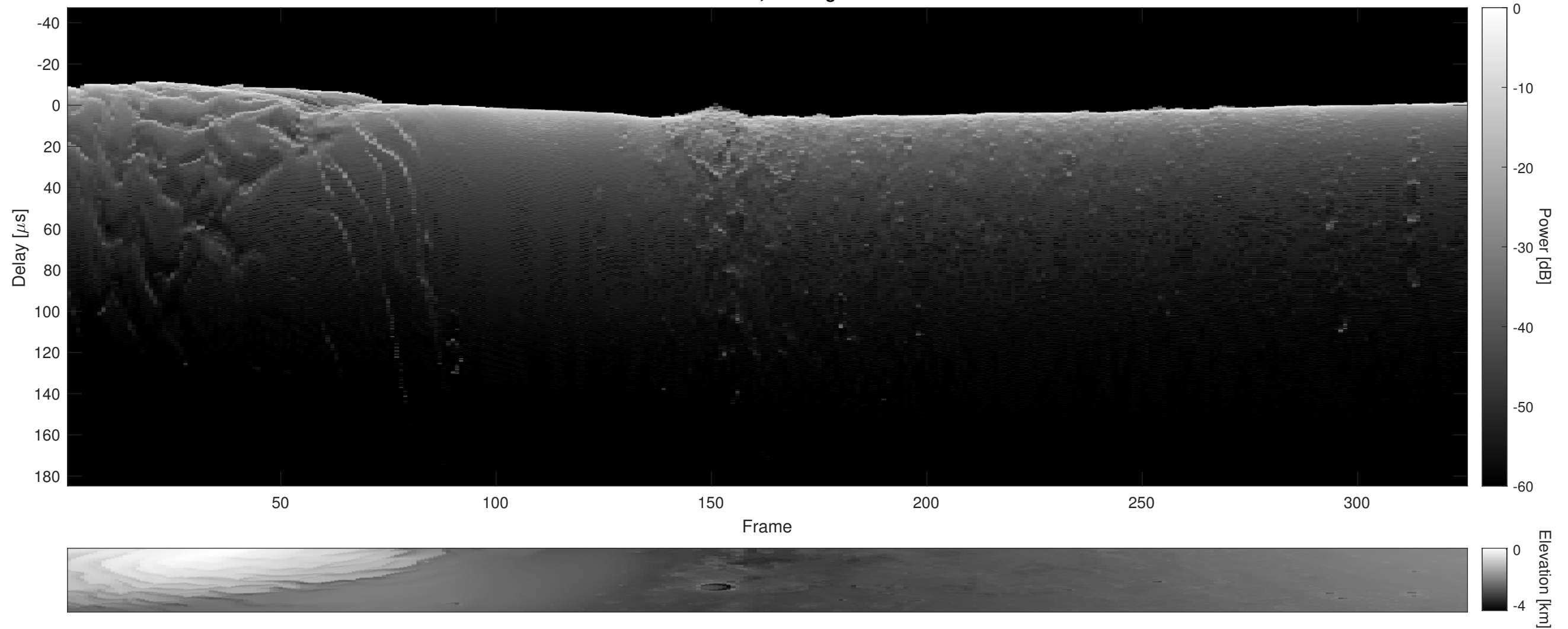
Orbit 13694, Cluttergram
