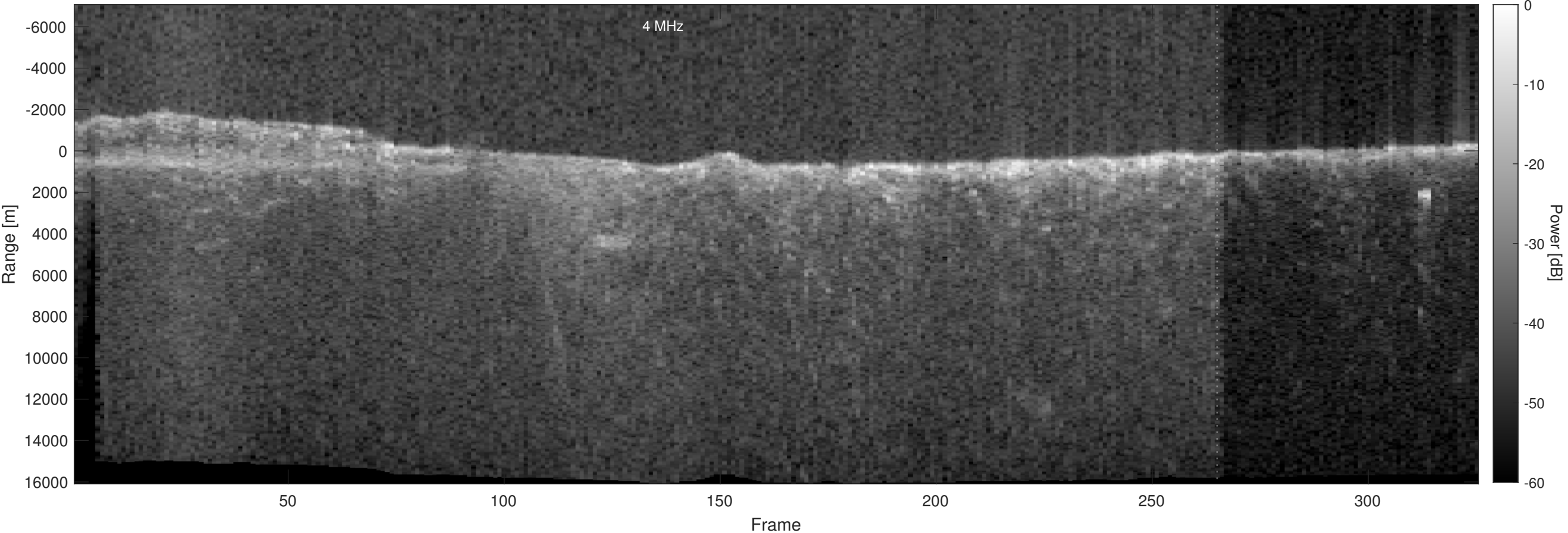
Orbit 13694, Optimized, Window, Depth-Corrected, Channel 2
