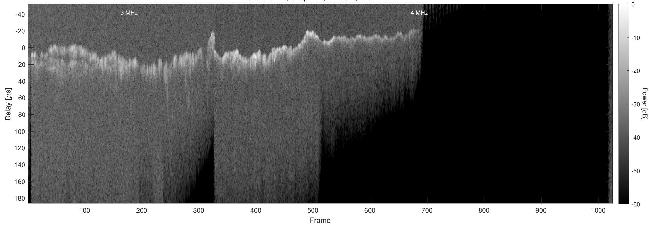
Orbit 13721, Chapman, Window, Channel 2
