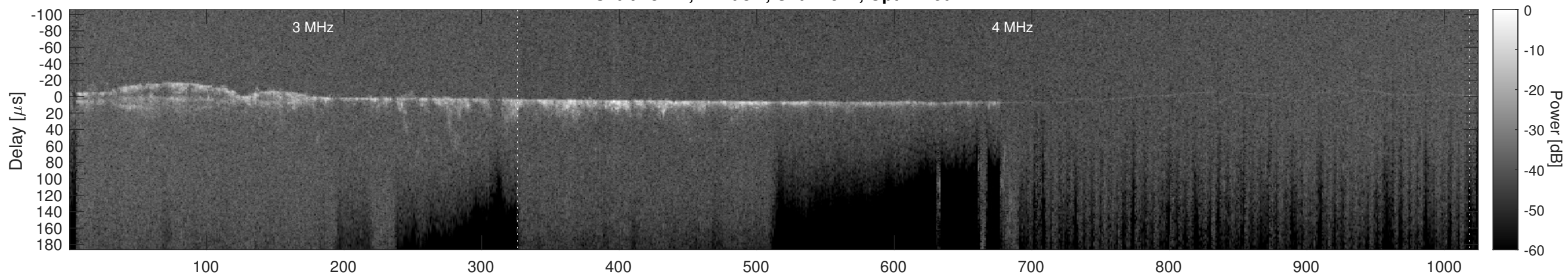
Orbit 13721, Cluttergram
