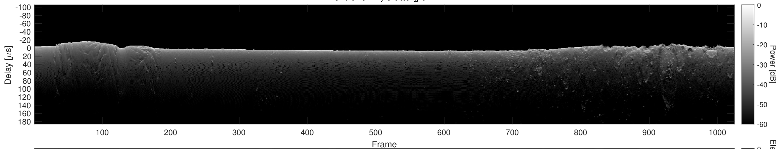
Orbit 13721, Cluttergram
