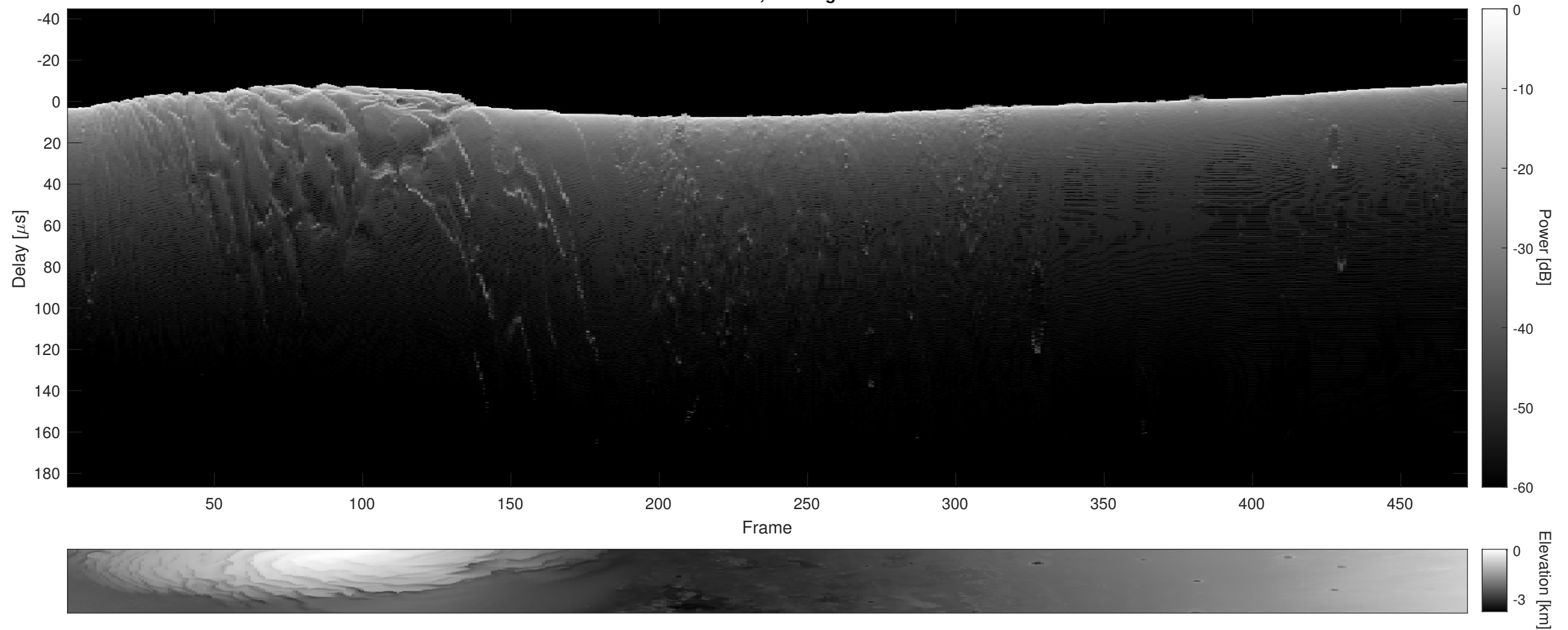
Orbit 13729, Cluttergram
