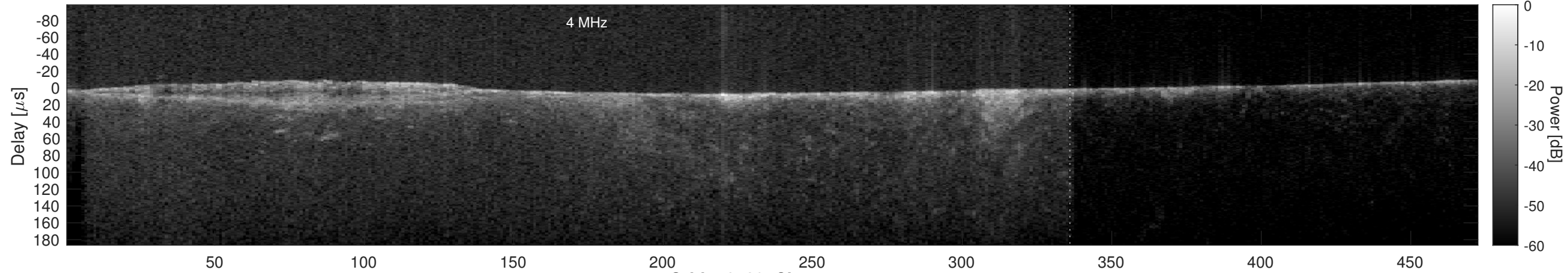
Orbit 13729, Cluttergram
